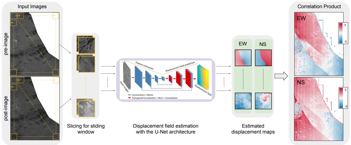
Fig. 1. Input satellite images are tiled up into large 256 \times 256 patches, processed into the CNN model, retrieving 256 \times 256 displacement fields, used to reconstruct full-scale full displacement maps.
