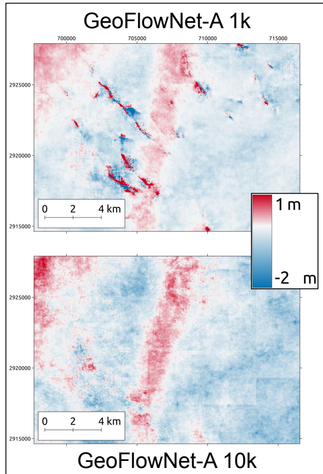
Fig. 10. 880 \times 1256 pixels crop of Balochistan displacement maps, for the two GeoFlowNet-A models trained with 4 \times 1k samples and a model trained with 4 \times 10k samples (respectively named GeoFlowNet-A 1k and GeoFlowNet-A 10k).
