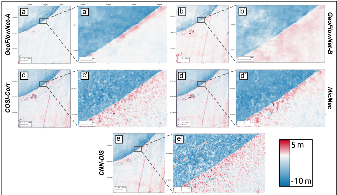
Fig. 8. EW component of the displacement maps from Landsat images for the Balochistan earthquake. From top to bottom: GeoFlowNet-A, GeoFlowNet-B, COSI-Corr, MicMac and CNN-DIS displacement maps (left column). A zoom on the Hoshab fault is shown on the right column for every method. Results are expressed in meters, with one pixel being 15 meters.
