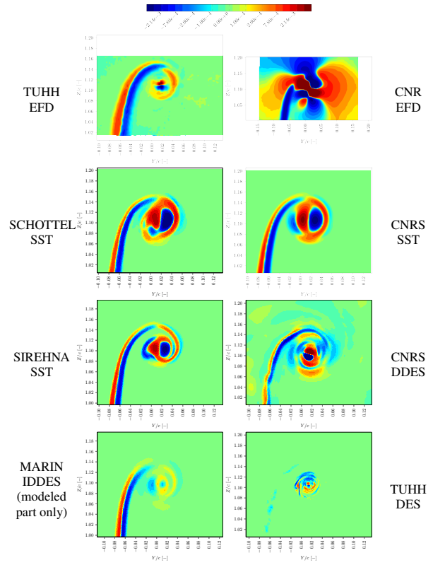
Figure 25: Reynolds Stress Tensor \overline{u'_x u'_y}
