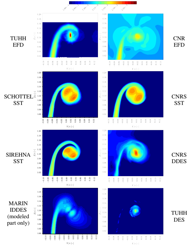
Figure 24: Reynolds Stress Tensor \overline{u'_z u'_z}
