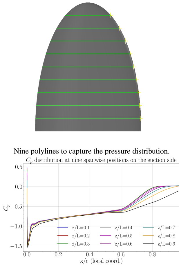
C_p distribution.
