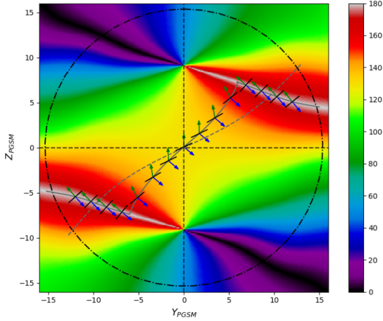
Figure 18. Global distribution of the magnetic shear ( ^{\circ} ) represented in panel a, using in-situ measurements for a IMF cone angle of 80^{\circ} \leq |\theta_{co}| \leq 90^{\circ} , an IMF clock angle has a value of 130^{\circ} , and a dipole tilt angle of \psi = 0^{\circ} \pm 2.5^{\circ} for the magnetosphere. The solid gray line is the MSL, along which the orientation of the magnetospheric and magnetosheath magnetic fields are indicated by the green and blue arrows, respectively. The small black lines correspond to the local bisections of the magnetic fields. The dashed gray line follow the local bisection of the magnetic fields, as integrated from the subsolar point.
