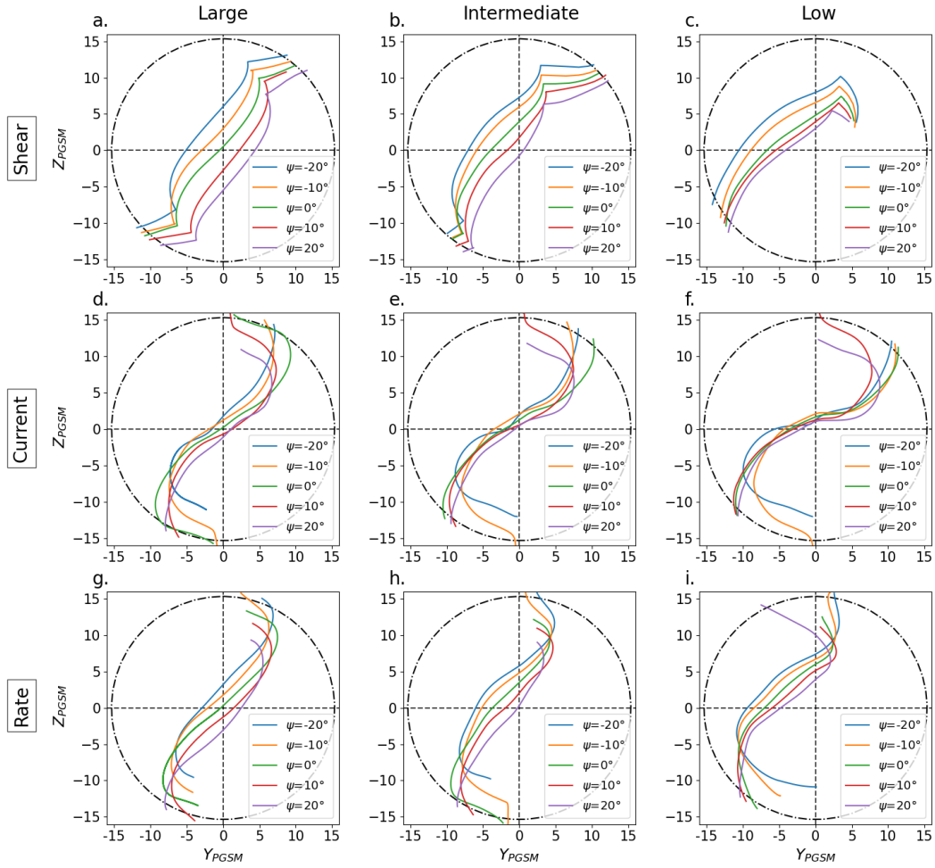
Figure 15. Lines maximizing the magnetic shear (panels a, b, c), the current density (panels d, e, f), and reconnection rate (panels g, h, i) at large (panels a, d, g), intermediate (panels b, e, h) and low (panels c, f, i) IMF cone angle and for an IMF clock angle of 60^\circ as a function of the dipole tilt angle ( -20^\circ , -10^\circ , 0^\circ , 10^\circ , and 20^\circ ). The dashed circle represents the terminator.
