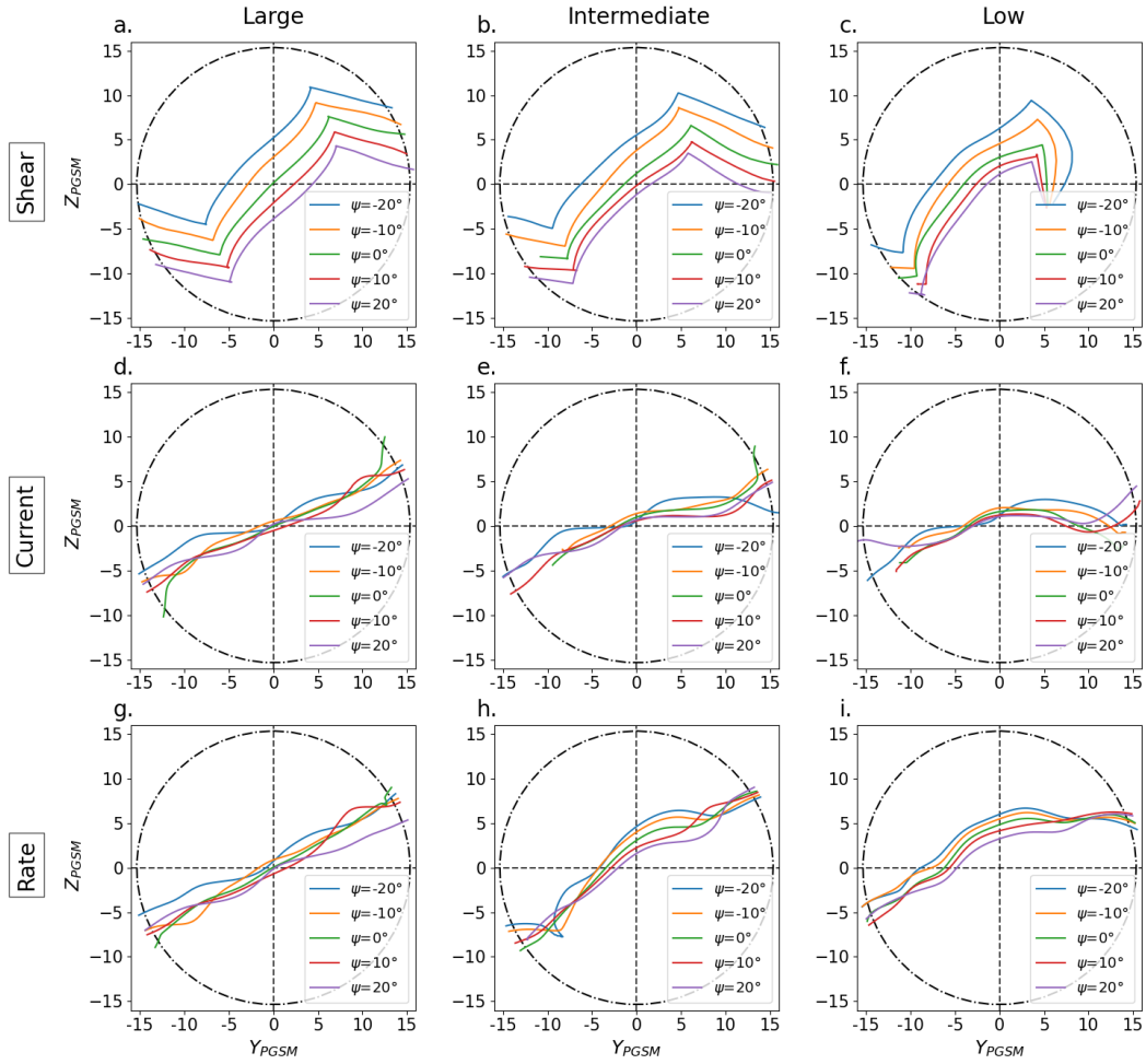
Figure 16. Lines maximizing the magnetic shear (panels a, b, c), the current density (panels d, e, f), and reconnection rate (panels g, h, i) at large (panels a, d, g), intermediate (panels b, e, h) and low (panels c, f, i) IMF cone angles and for an IMF clock angle of 120^\circ as a function of the dipole tilt angle ( -20^\circ , -10^\circ , 0^\circ , 10^\circ , and 20^\circ ). The dashed circle represents the terminator.
