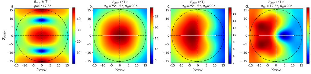
Figure 10. Amplitude of the magnetic fields at the surface of the magnetopause. Panel a shows the distribution of the magnetospheric magnetic field strength for a dipole tilt angle of \psi = 0^\circ \pm 2.5^\circ . Panels b, c, and d show the amplitude of the magnetosheath magnetic field for large ( 70^\circ \leq |\theta_{co}| \leq 80^\circ ), intermediate ( 20^\circ \leq |\theta_{co}| \leq 30^\circ ), and small ( |\theta_{co}| \leq 12.5^\circ ) IMF cone angle and an IMF clock angle of 90^\circ , respectively.
