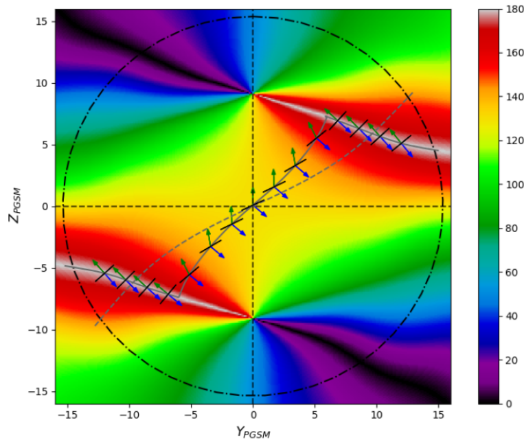
Figure 18. Global distribution of the magnetic shear ( ^{\circ} ) represented in panel a, using in-situ measurements for a IMF cone angle of 80^{\circ} \leq |\theta_{co}| \leq 90^{\circ} , an IMF clock angle has a value of 130^{\circ} , and a dipole tilt angle of \psi = 0^{\circ} \pm 2.5^{\circ} for the magnetosphere. The solid gray line is the MSL, along which the orientation of the magnetospheric and magnetosheath magnetic fields are indicated by the green and blue arrows, respectively. The small black lines correspond to the local bisections of the magnetic fields. The dashed gray line follow the local bisection of the magnetic fields, as integrated from the subsolar point.
