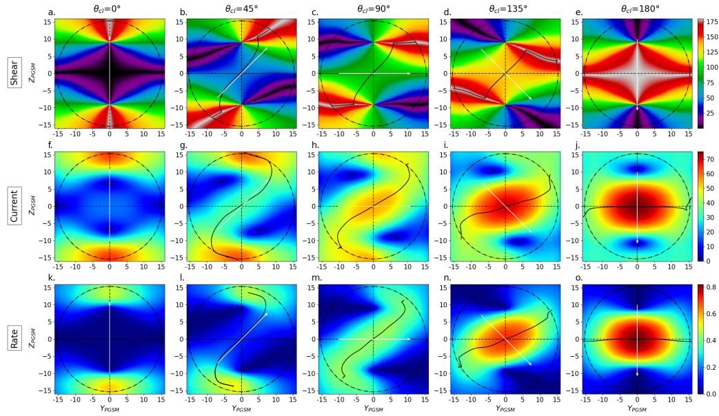
Figure 11. Global distributions of magnetic shear ( ^\circ ), current density ( nA/m^2 ), and reconnection rate ( mV/m ) at the surface of the magnetopause at Large IMF cone angles. Subsets of the measurement for IMF cone angles in the range 70^\circ \leq |\theta_{co}| \leq 80^\circ and dipole tilt angles of |\psi| = 0^\circ \pm 2.5^\circ . The magnetic shear (panels a to e), the current density (panels f to j), and the reconnection rate (panels k to o) for IMF clock angle 0^\circ (panels a, f, and k), 45^\circ (panels b, g, and l), 90^\circ (panels c, h, and m), 135^\circ (panels d, i, and n), and 180^\circ (panels e, j, and o). The black lines maximize the quantities represented in each panel. The white arrows correspond to IMF orientation in the (YZ) plane. The terminator is represented by the dashed circle.
