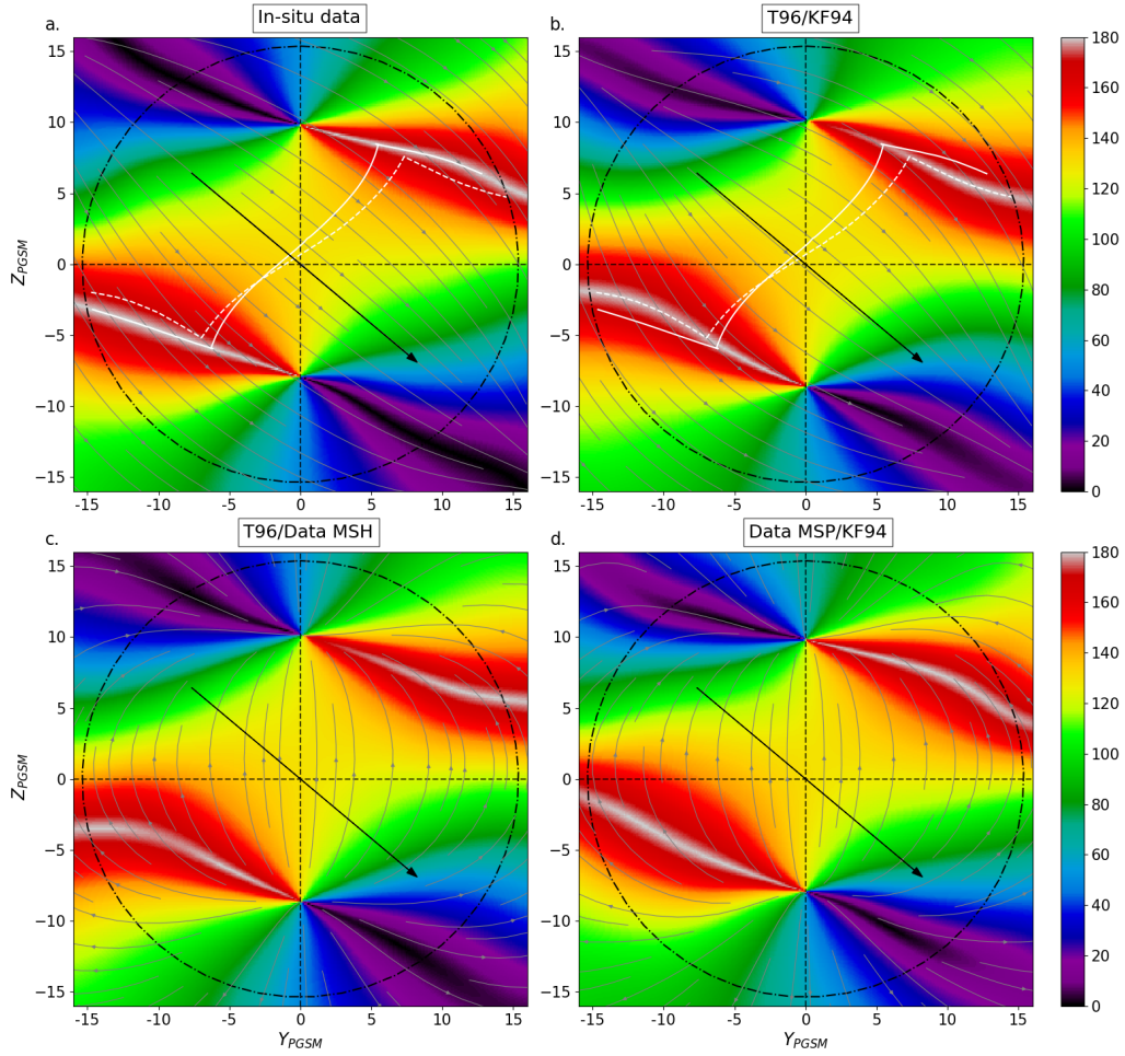
Figure 5. Magnetic shear maps at large IMF cone angle. Panels a and b correspond to the magnetic shear angle in degrees ( ^{\circ} ) using only in-situ measurements and magnetic field models Tsyganenko & Stern (1996); Kobel & Fluckiger (1994), respectively. The magnetic shear map on panel b correspond to the one presented in Trattner et al. 2021Trattner et al. (2021) (Fig.13) on 20 September 1997 at 07:34 UT. The map in panel c is made with the T96 model and the magnetosheath in-situ measurements. The map in panel d is made with the magnetosphere in-situ measurements and the KF94 model. The subset of in-situ magnetosheath measurements used in panels a and c is 76^{\circ} \leq |\theta_{co}| \leq 86^{\circ} and turned to an IMF clock angle of 130^{\circ} . The subset of in-situ magnetosphere measurements used in panels a and d is |\psi| = 6.6^{\circ} \pm 2.5^{\circ} . The value of dipole tilt of modeled magnetospheric magnetic field (Tsyganenko & Stern (1996)) used in the panels b and c is -6.6^{\circ} . The modeled magnetosheath magnetic field (Kobel & Fluckiger (1994)) in the panels b and d is made with (Bx_{imf}, By_{imf}, Bz_{imf}) = (-0.7, 3.8, -3.2) . The grey arrowed lines in the panels a and b (resp. c and d ) represent magnetic field lines of the observed and modeled magnetosheath (resp. magnetosphere), respectively. The solid and dashed white lines maximize the observed and modeled magnetic shear, respectively. The black arrows correspond to IMF orientation in the (YZ) plane. The terminator is represented by the dashed circle.
