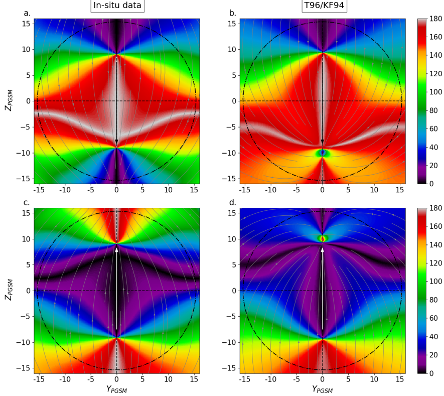
Figure 7. Magnetic shear ( ^{\circ} ) maps at intermediate IMF cone angle. Subsets \theta_{co} = 25^{\circ} \pm 5^{\circ} and |\psi| = 0^{\circ} \pm 2.5^{\circ} with \theta_{cl} = 180^{\circ} (Panel a and b) and \theta_{cl} = 0^{\circ} (Panel c and d). The legend is the same as Figure 6.
