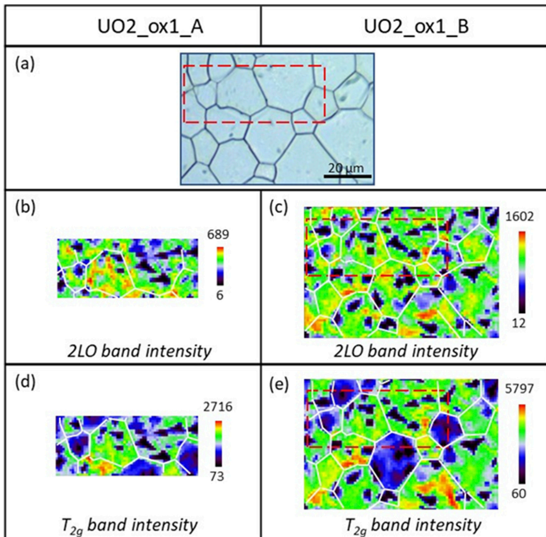
FIGURE 2 Raman mapping of the 2LO and T 2g band intensities at the surface of sample UO 2 _ox1 after two oxidations (samples UO 2 _ox1_A on the left and UO 2 _ox1_B on the right). (A) Optical picture of the analyzed region; (B) and (C) Raman mapping of the 2LO band intensity; (D) and (E) Raman mapping of the T 2g band intensity. The color scale corresponds to the intensity scale, from the lowest (black) to the highest (red) value. For clarity, grain boundaries visible on the optical picture are represented by white lines on the mapping.
