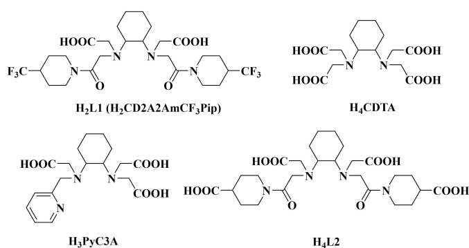
Scheme 1. Ligand structures.
