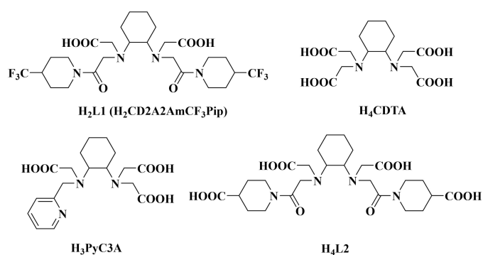
Scheme 1. Ligand structures.
