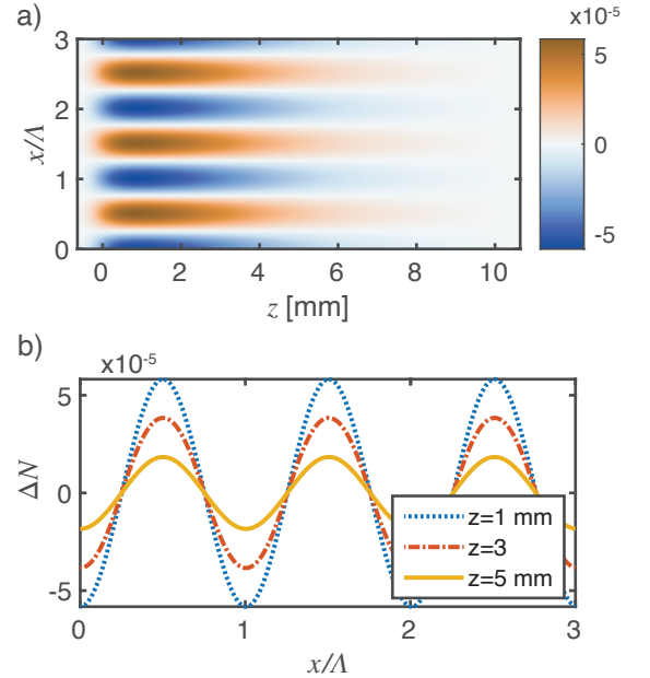
FIG. 5. Refractive index modulation (i.e., optical grating) created at t = \tau_s/2 with the same conditions as the previous figures ( 60 \text{ mJ/cm}^2 of average UV fluence and 2% ozone concentration). a) Index modulation \Delta n(x, z) ; b) lineouts along x taken at z = 1, 3 and 5 mm.
