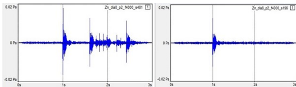
Figure 3: Temporal evolution of two audio stimuli as examples of crack-like sounds heard during the slip audio events.
