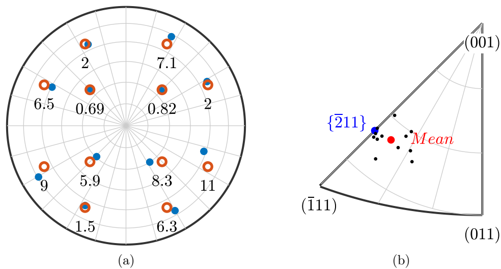
Fig. 9. Comparison between Pitsch invariant direction and computed lath normals in the parent frame. (a) Element-wise variant comparison. The computed directions are plotted as blue points, and \{\bar{2}11\} equivalent directions as red circles. The angular error between both directions is indicated for each variant in degrees. (b) Comparison between the equivalent average pole and direction. The twelve computed poles are represented as black points. The average distance between measured and computed poles is 4.1^\circ
