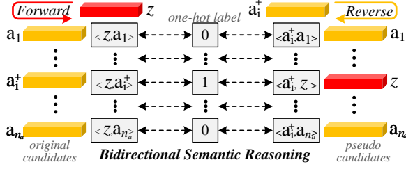
Fig. 4. The proposed BSR learning paradigm. It encourages the model to flexibly build the positive correlation from the predicted feature to the ground-truth answer while suppressing spurious correlations to all negative candidates without a prespecified margin via forward semantic reasoning (left). And it widens the semantic gap between the positive answer and all negative candidates to strengthen the unique positive semantic correlation from the positive answer to the predicted feature via reverse semantic reasoning (right).
