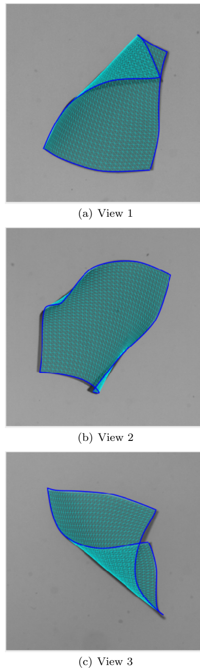
Fig. 11 Reprojection of the optimized mapped model perimeter [ — ] and mapped model mesh [ ■ ] for a square sheet particle. The cropped region is 343 px \times 343 px in size
