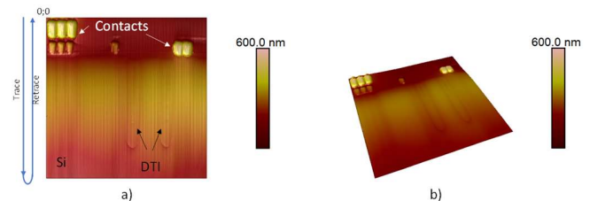
Figure 3: Topography of the studied device (cross-sectional preparation) a) 2D and b) 3D view.
