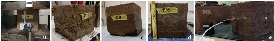
FIGURE 2. Compressive strength (a-b); water capillary absorption (c-d); thermal conductivity (e) tests for RE materials.
