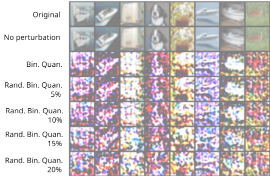
Fig. 3: Data reconstruction under different perturbation levels. Row 1 is the original input image, row 2 is the data reconstruction without perturbation, rows 3-7 are data reconstruction with different levels of randomized binary quantization.
