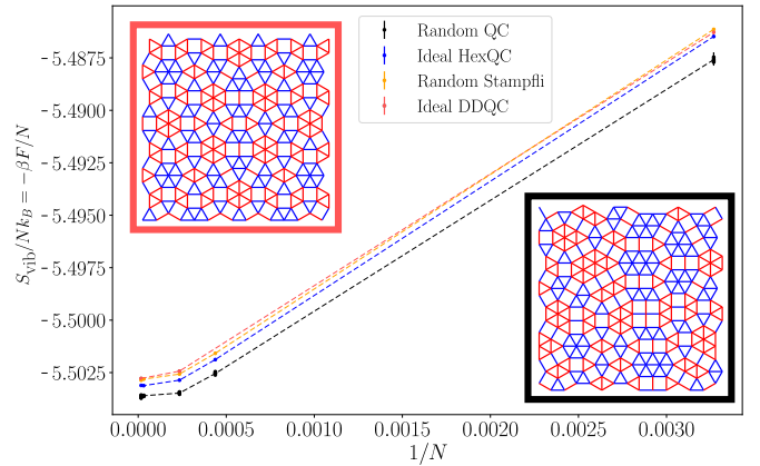
FIG. 2: Vibrational entropies of the Schlottmann (dodecagonal, pink), random Stampfli (dodecagonal, orange), Stampfli (hexagonal, blue) and 5 fully random quasicrystals (dodecagonal, black), for various system size. The error bars are the statistical error on the mean obtained by repeating Frenkel-Ladd calculations many times, and are smaller than the symbols for most points. Two system sizes are obtained by inflation of a sigma seed, for which our implementation of the Schlottmann inflation fails. Hence, two pink points are missing. The inset show examples of an ideal Schlottmann tiling (bottom left) and a random tiling (upper right).
