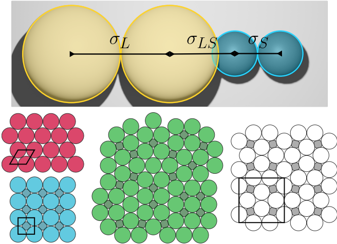
FIG. 1: (Top) Schematic image of binary hard spheres lying on a flat plane. The line segments indicate the contact distances for the different species. (Bottom) Candidate phases considered for this system: hexagonal packing (red), S1 (blue), QC12 (green) and Sigma (white). The unit cell of the periodic structures are depicted as black rhombi.
