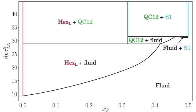
FIG. 4: Phase diagram of binary mixtures of non-additive hard disks with size ratio q = 0.46 corresponding to the equivalent 3D geometry of spheres sedimented on a flat surface. The random tiling dodecagonal quasicrystal is labelled “QC12”. Although considered as a candidate phase, the Sigma approximant of the quasicrystal is nowhere stable.
