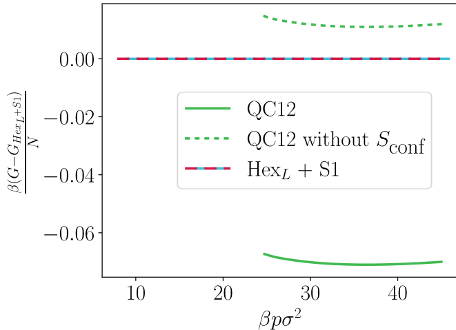
FIG. 3: Free-energy difference between the competing coexistence of \text{Hex}_L + \text{S1} and the quasicrystal at the quasicrystal composition. For the quasicrystal, the dashed curve corresponding to the vibrational entropy alone and lies above the coexistence free-energy, while the addition of the constant tiling entropy term (solid line) stabilizes the quasicrystal.
