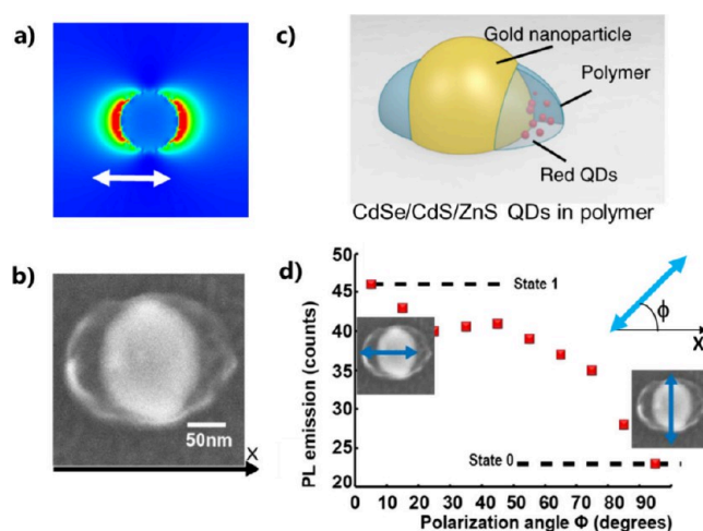
Figure 10. D_{\infty h} symmetry of a gold nanodisk leads to D_{2h} symmetry of the active medium by Plasmonic two-photon polymerization (P2PP) using linear polarization. (a) FDTD calculation of the intensity of the near-field, used for P2PP, of the nanodisks at \lambda = 780 nm. The white arrow represents the direction of polarization used for P2PP. (b) SEM image of the resulting HPN: Au nanodisk surrounded by two polymer lobes containing QDs. (c) Illustration of the hybrid nanosystem. (d) Photoluminescence intensity from the hybrid structure as a function of \phi ; the angle of polarization of the exciting linearly polarized laser beam at 405 nm wavelength. The figure on the right represents the X -axis, \phi , and the linear polarization used for post characterization. (a–d) Adapted with permission from ref 3 under Creative Commons CC BY license. Copyright 2020 The Author(s).
