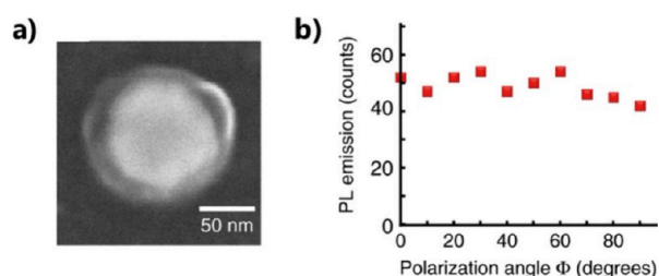
Figure 11. D_{\infty h} symmetry of a gold nanodisk transferred to the active medium by P2PP using circular polarization. (a) SEM image of a gold nanodisk surrounded by a polymer ring containing QDs. (b) Photoluminescence from the hybrid structure, excited with a linearly polarized laser beam at 405 nm wavelength, as a function of the polarization in-plane angle \phi . (a, b) Adapted with permission from ref 3. Copyright 2020 The Author(s) under Creative Commons CC BY license.
