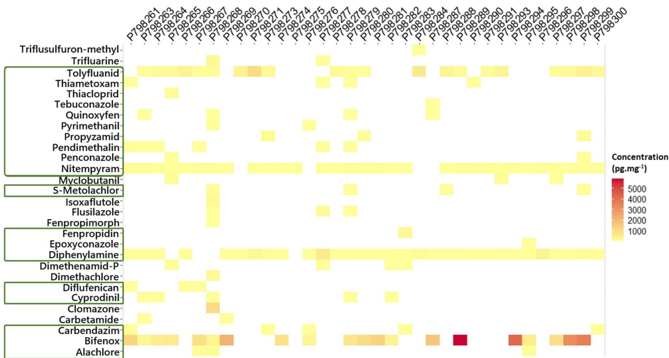
Fig. 2 Heat map illustrating the concentration (pg.mg -1 ) of the 29 pesticide molecules found in the blood of 35 captive grey partridges. The redder the concentration, the higher the concentration. The molecules framed in green are those also found in wild partridges
