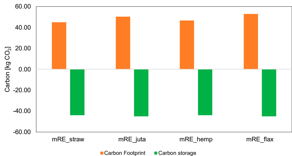
Figure 10. Carbon footprint and carbon storage of the mRE system for different natural fibers used in the raw earth mixture.
