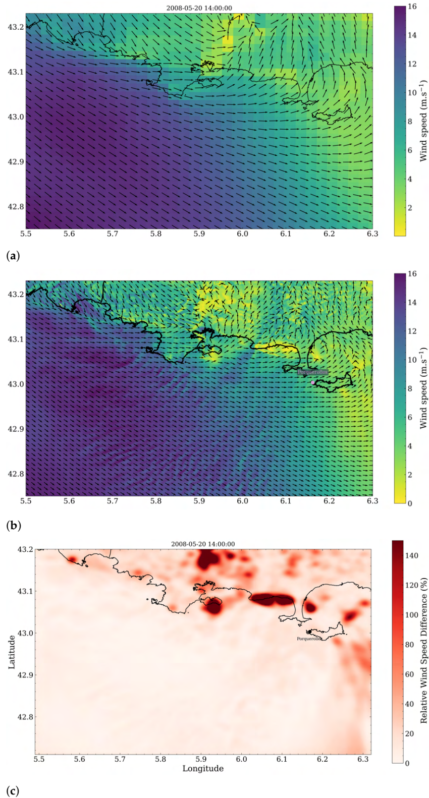
Figure 5. Wind field calculated for the day of 20 May at 2 p.m. using the Meso-NH model where panel (a) shows the simulations made using the kilometric resolution, (b) the LES calculations and (c) the relative difference of the wind speed calculated by the two models. Note: The arrows indicating wind direction arrows do not indicate wind speed magnitude.
