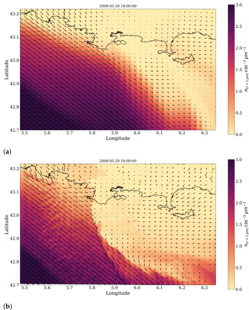
Figure 11. Map of sea-spray concentration calculated using the MesoNH (a) and the MesoNH LES (b) model for the day of 20 May at 6 p.m.
