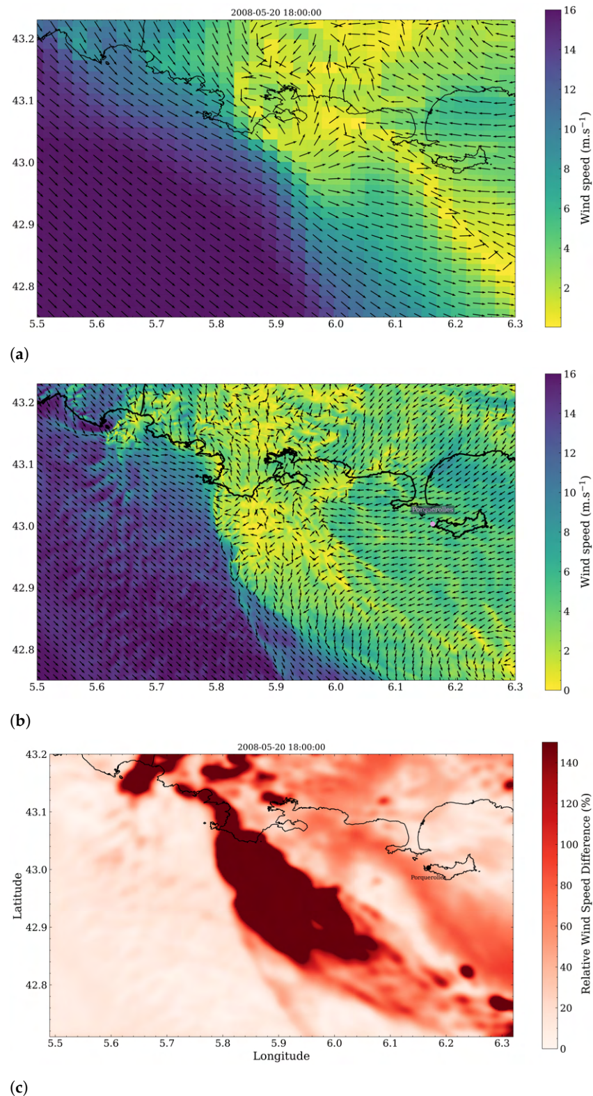
Figure 4. Wind field calculated for 20 May at 6 p.m. using the Meso-NH model. Panel (a) shows the simulations made using kilometric resolution, (b) the LES calculations and (c) the relative difference in wind speed calculated by the two models. Note: The arrows indicating wind direction arrows do not indicate wind speed magnitude.
