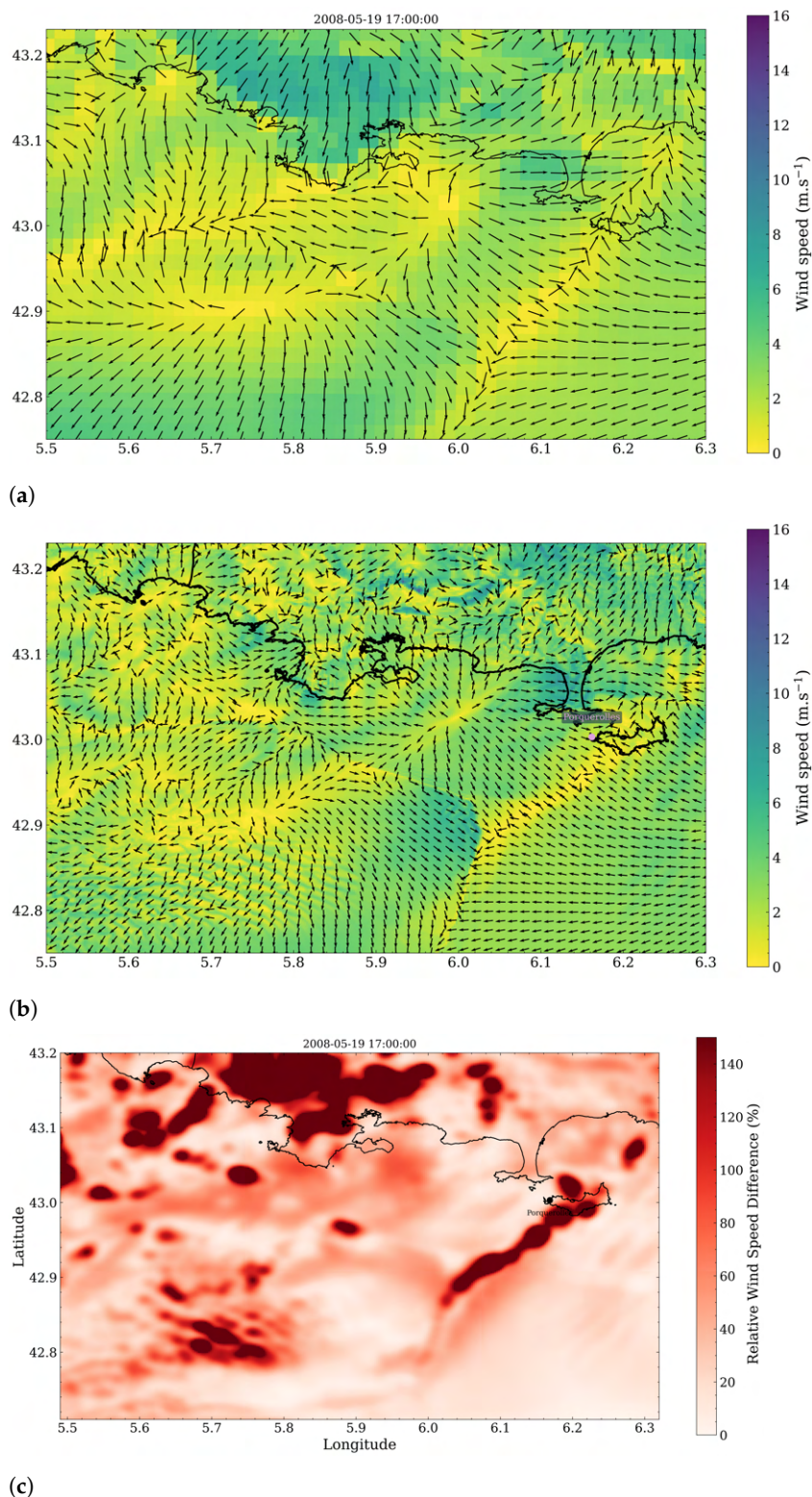
Figure 6. Wind field calculated for the day of 19 May at 5 p.m. using the Meso-NH model. Panel (a) shows the simulations made using the kilometric resolution, (b) the LES calculations and (c) the relative difference of the wind speed calculated by the two models. Note: The arrows indicating wind directions are not proportional to wind speed.
