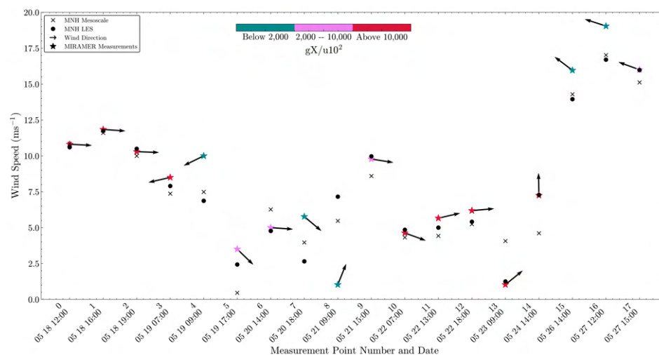
Figure 7. A comparison of the wind speed measurements taken on board the R/V Atalante (stars symbols) with the numerical simulations from both the mesoscale model (crosses) and the high-resolution model (bullets). The numbers on the x-axis correspond to the measurements points as shown in Figure 1. The colour of the stars indicates the calculated non-dimensional fetch (Equation (1)) as shown in the horizontal colour bar reported on the top of the figure. We also reported the wind direction recorded during each episode.
