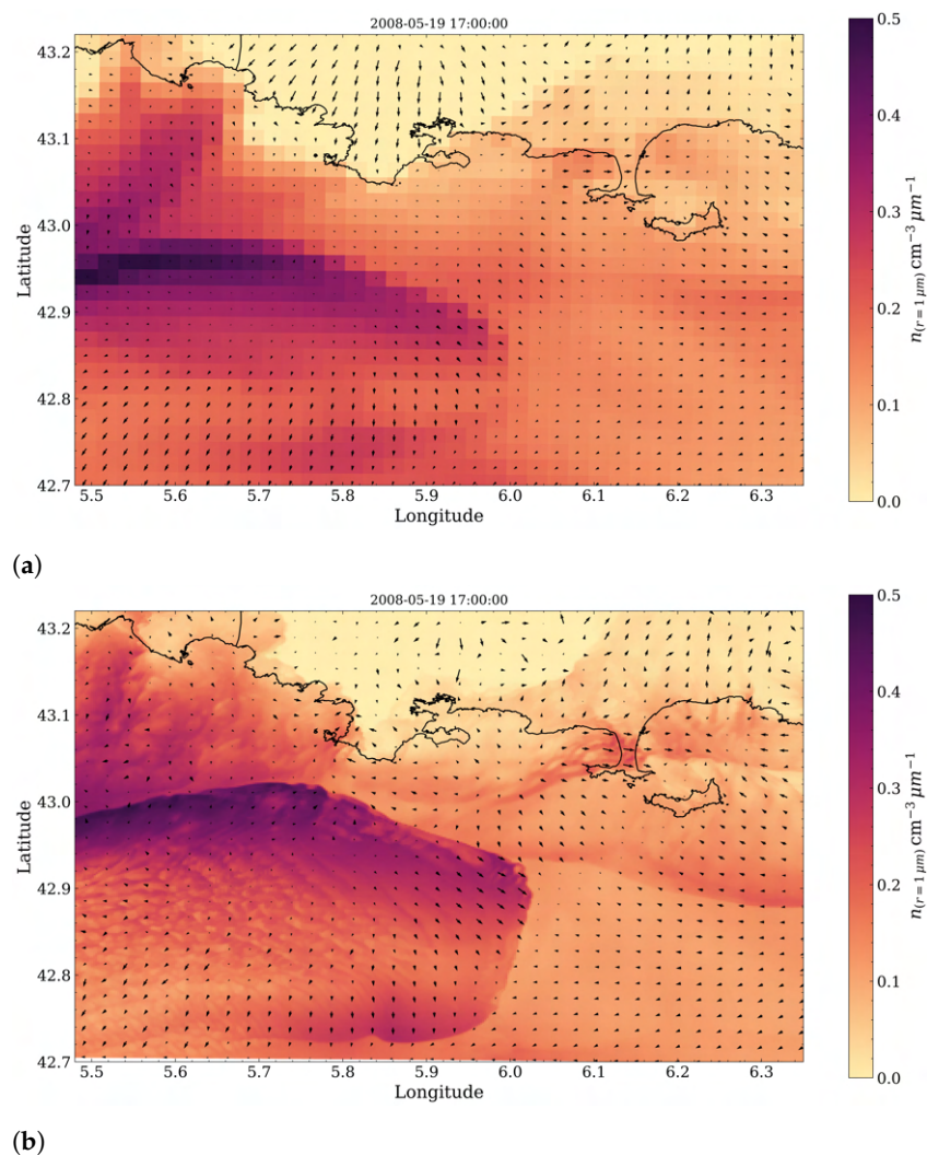
Figure 13. Map of sea-spray concentration calculated using the MesoNH (a) and the MesoNH LES (b) model for the day of 19 May at 5 p.m.
