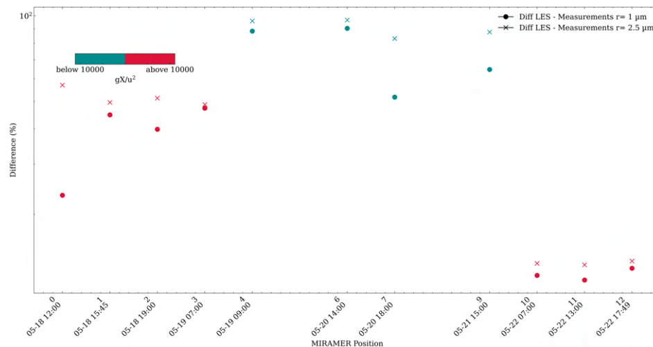
Figure 14. Difference between modeled and available observed aerosol concentrations, as measured on board the R/V Atalante, for selected radii of 1 \mu\text{m} (bullets) and 2.5 \mu\text{m} (crosses). Blue symbols correspond to non-dimensional fetch less than 10,000, red symbols correspond to non-dimensional fetch greater than 10,000.
