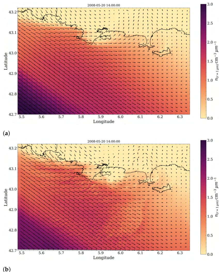
Figure 12. Map of sea-spray concentration calculated using the MesoNH (a) and the MesoNH LES (b) model for the day of 20 May at 2 p.m.
