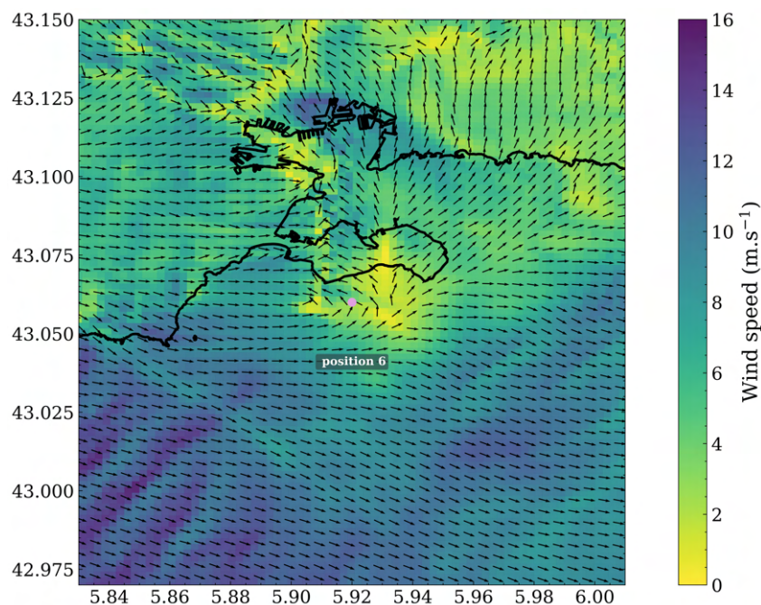
Figure 8. Zoom on the west portion of Figure 5b. The pink dot indicates the location of the measurements. Note: The arrows indicating wind directions are not proportional to wind speed.
