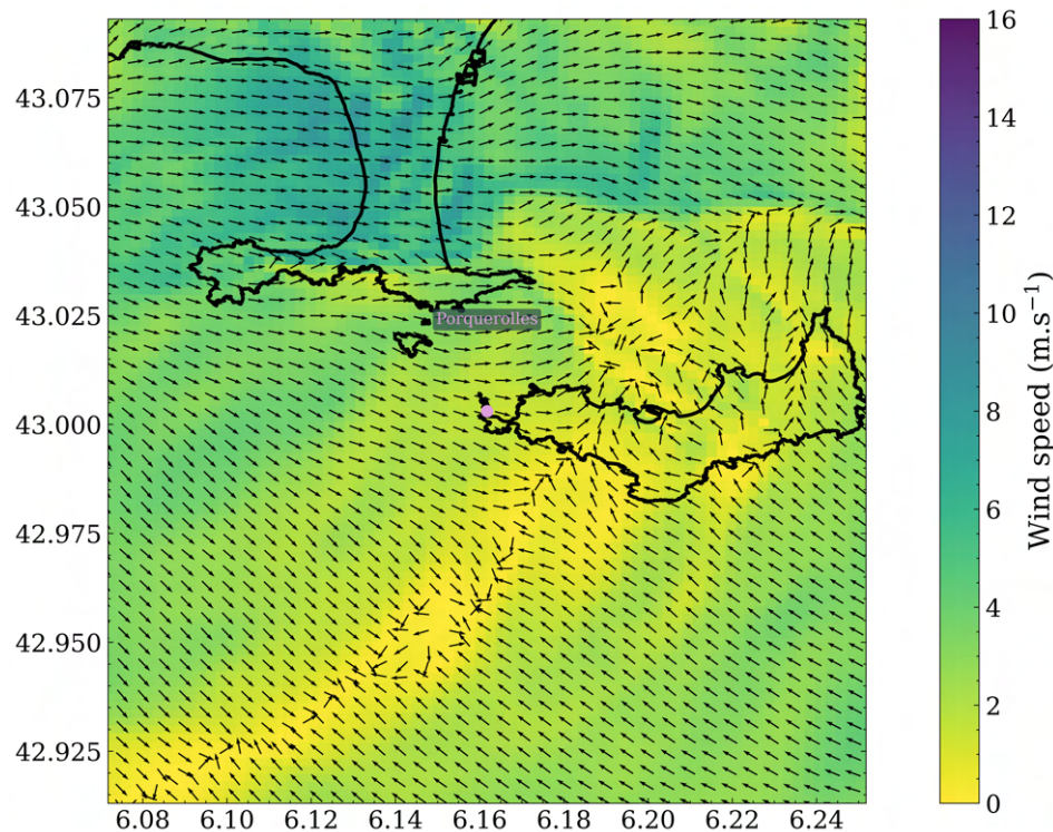
Figure 9. Zoom on east portion of Figure 6b. The pink dot indicates the location of the measurements. Note: The arrows indicating wind directions are not proportional to wind speed.
