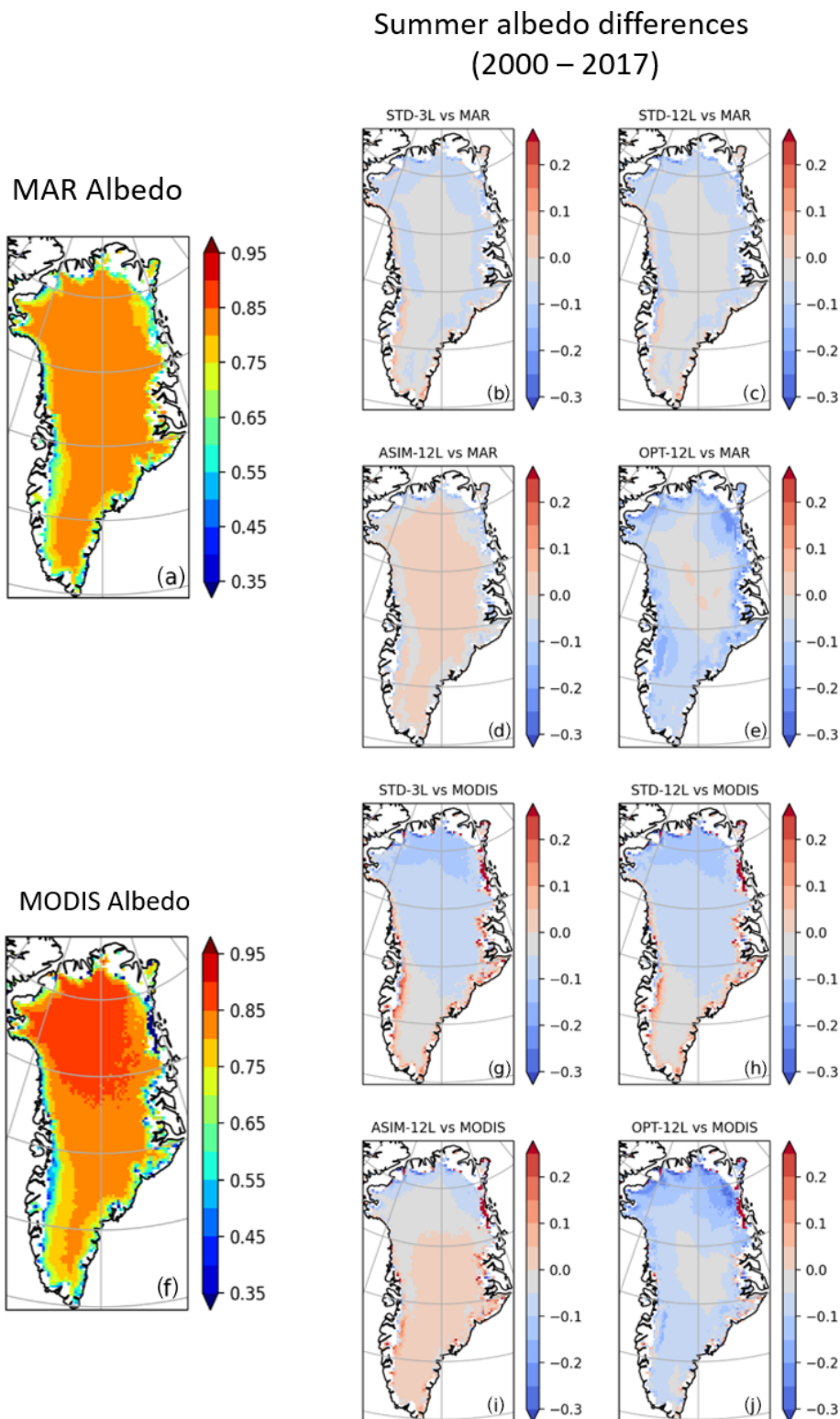
Figure 6. Left – spatial distribution of the summer (JJA) albedo computed with MAR (a) and MODIS (f) and averaged over the 2000–2017 period. Right – differences between the albedo computed with ORCHIDEE-ICE and MAR (b–e) and between ORCHIDEE-ICE and MODIS (g–j) for the 3-layer snow scheme and the standard albedo parameters (b, g), the 12-layer snow scheme and the standard albedo parameters (c, h), the albedo parameters inferred from a data assimilation technique and using a previous version of the ORCHIDEE-ICE model (d, i), and the albedo parameters obtained after manual tuning (e, j).
