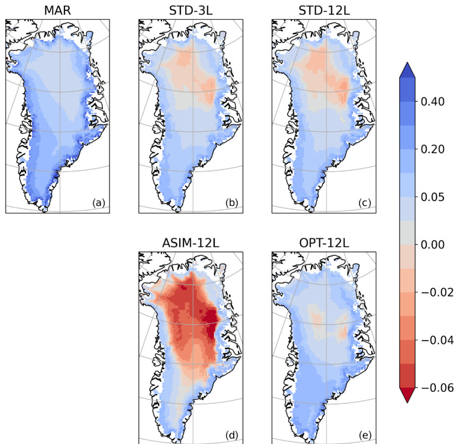
Figure 4. Same as Fig. 2 but for the simulated sublimation (in \text{mm d}^{-1} ). Negative values indicate condensation.
