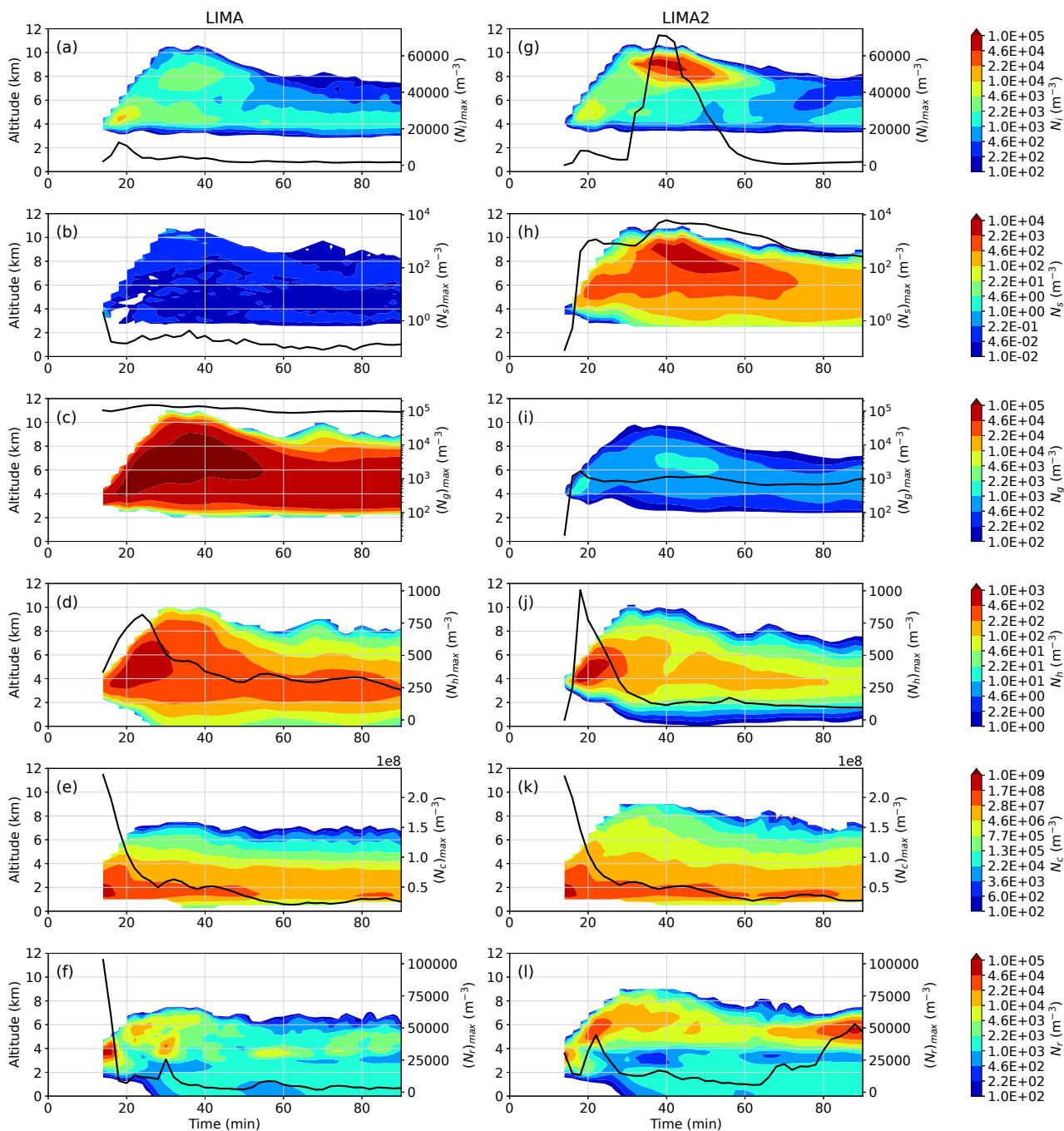
Figure 7. Same as Figure 6 with hydrometeor number concentrations.
