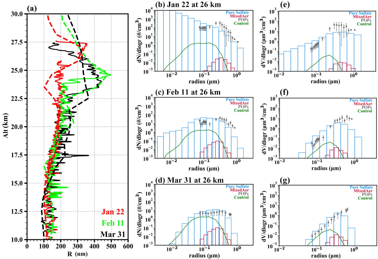
Figure 1. Comparison of the aerosol size with balloon-borne observations. (a) Observations of the aerosol effective radius (unit: nm) inside of the volcanic plume from the portable optical particle spectrometers (POPs) launched in Réunion Island (21°S, 55.4°E) on January 22, February 11 and March 31 of 2022 are denoted by solid lines. Simulated daily mean vertical distributions of aerosol effective radius inside the plume located near Réunion Island on the three balloon launch days are denoted by the dashed lines. (b–d) Comparison of the simulated aerosol number size distributions ( dN/d\log r , unit: \#/cm^3 ) with balloon observations (denoted by the black filled circles) at 26 km (Asher et al., 2023) on the three balloon launch days shown in each panel, respectively. Simulated aerosol number size distributions for the pure sulfate and mixed aerosols (detailed model settings in Section 2 and Yu et al., 2015) are denoted by the blue and red boxes, respectively. The simulated pure sulfate number size distributions on each balloon launch day without HTHH eruption are denoted by the green solid lines in each panel, respectively. Panels (e–g) same as panels (b–d) but for volume distribution ( dV/d\log r , unit: \mu m^3/cm^3 ).
