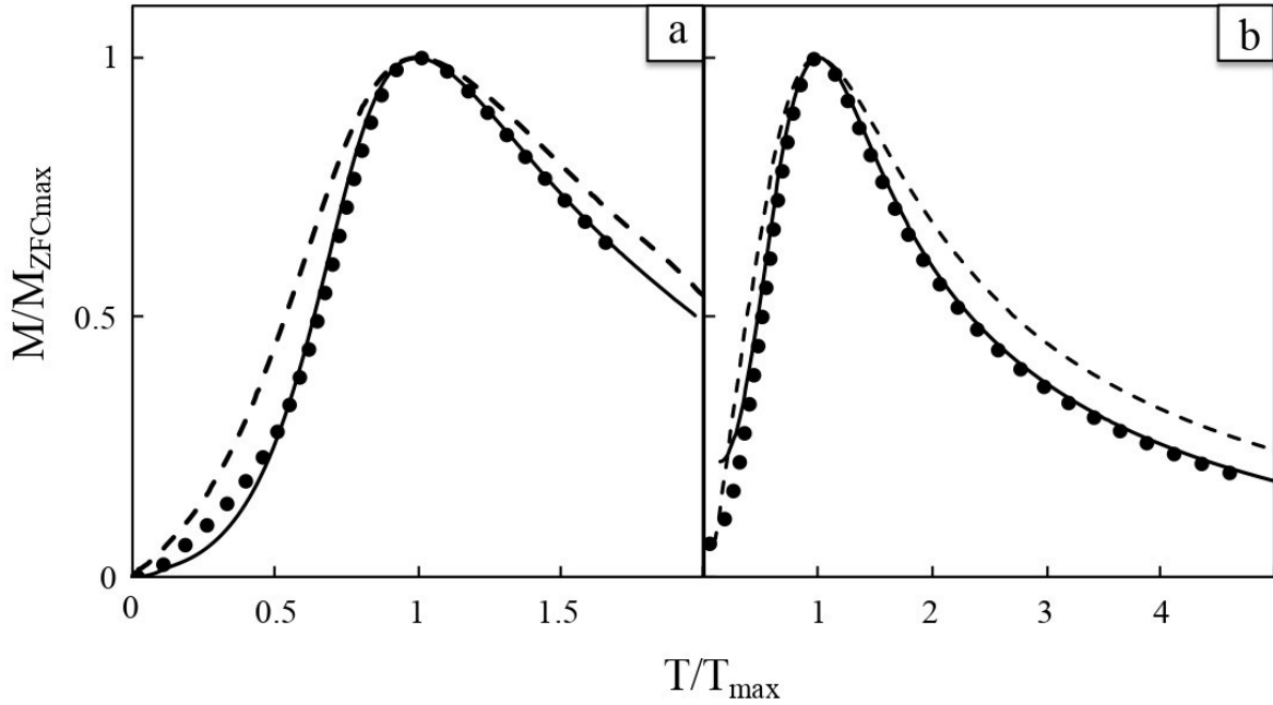
Figure 5. Zero field magnetization versus temperature curves normalized to T_{\max} of maghemite nanoparticles synthesized from iron oleate (solid line), iron dodeconoate (full circles), and iron octanoate (dashed line). (a) large-nanoparticle sizes, (b) intermediate-nanoparticle sizes.
