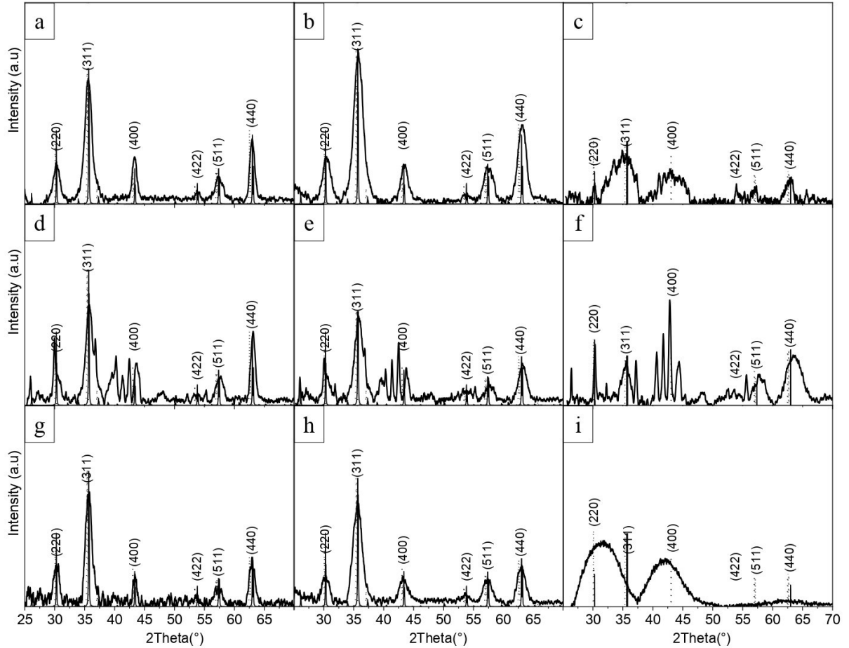
Figure 3. X-ray diffraction (XRD) patterns of iron oxide nanoparticles synthesized from (a,b,c) iron oleate, (d,e,f) iron dodeconoate, and (g,h,i) iron octanoate. The mean diameters are centered on (a,d,g) 12.0 nm, (b,e,g) 7.5 nm and (c,f,i) 3.3 nm. Solid lines: maghemite (Ref. 04-021-3968, PDF-5) reference pattern. Dotted lines: magnetite (Ref. 04-027-0607, PDF-5) reference patterns.
