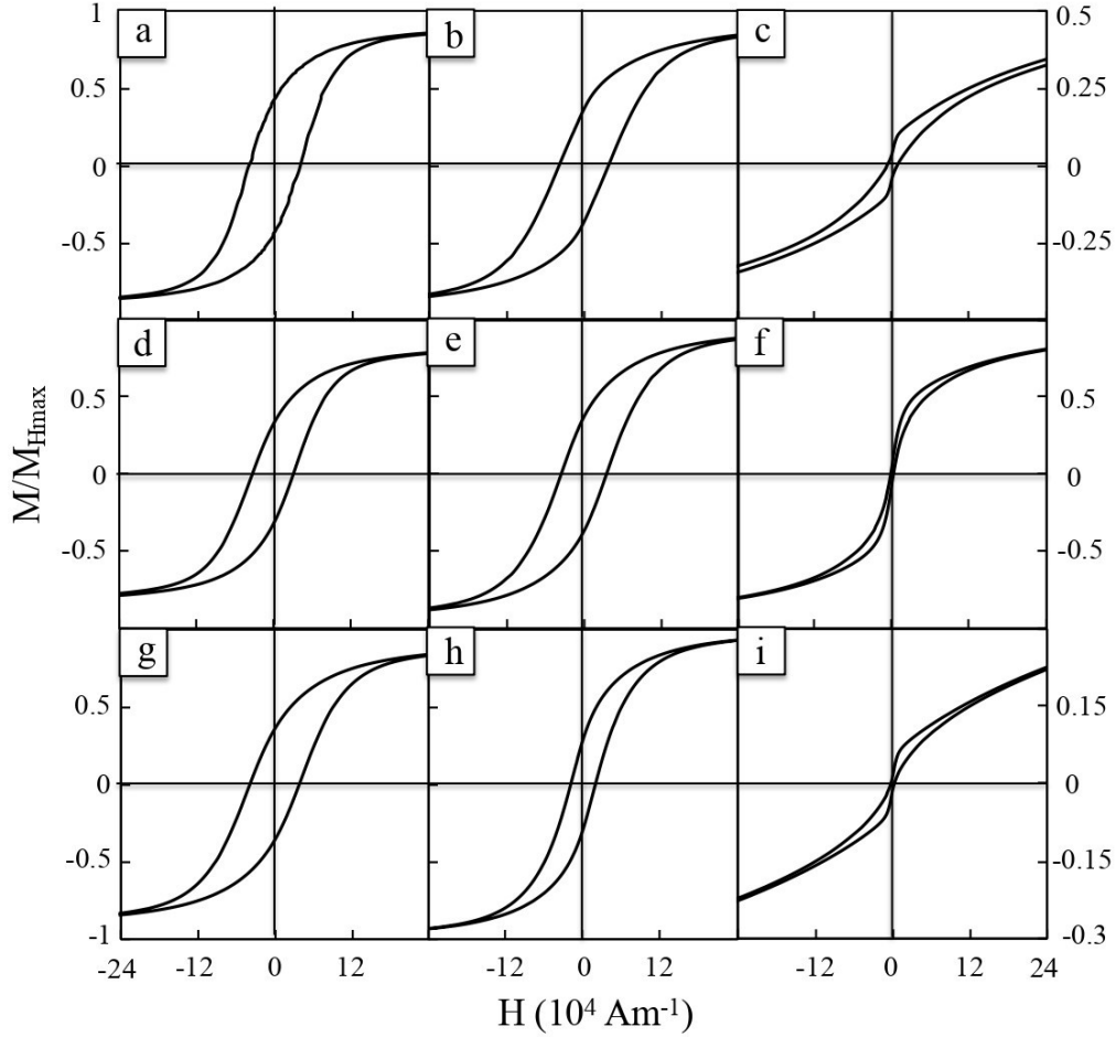
Figure 6. Hysteresis curves performed at 3 K, of maghemite nanoparticles synthesized from (a,b,c) iron oleate, (d,e,h) iron dodecanoate, and (g,h,i) iron octanoate. The mean diameters are centered on (a,d,g) 12.0 nm, (b,e,g) 7.5 nm and (c,f, i) 3.3 nm.
