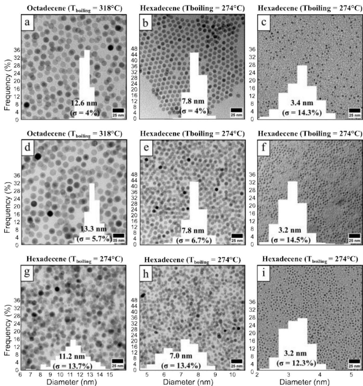
Figure 2. Transmission electron microscopy (TEM) images of maghemite nanoparticles synthesized from (a,b,c) iron oleate, (d,e,f) iron dodeconoate, and (g,h,i) iron octanoate. The mean diameters are centered on (a,d,g) 12.0 nm, (b,e,g) 7.5 nm and (c,f,i) 3.3 nm.
