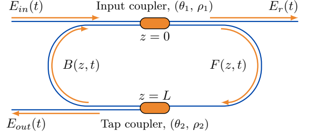
FIG. 2. The Fabry-Perot cavity of Fig. 1 in the limit G = 0 is equivalent to a ring cavity composed of two identical pieces of fibers of length L connected by two couplers (\theta_1, \rho_1) and (\theta_2, \rho_2) .
