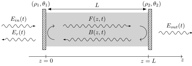
FIG. 1. Schematic diagram of a nonlinear FP cavity of arbitrary finesse located in the interval 0 \leq z \leq L .
