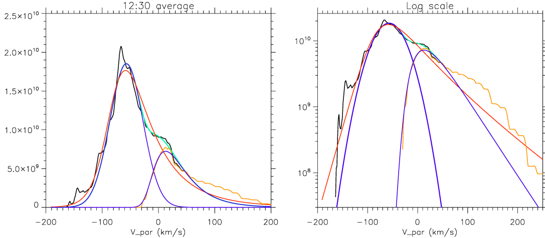
Fig. 4. Average distribution at 12:30 (same as in Fig. 3). The Gaussian fit of the core ( M_c ) and the NIG fit of the beam (NigB) are shown in blue. M_c + \text{NigB} , almost undiscernible from the measured distribution, is shown in green. The NIG fit of the whole distribution (NigT) is shown in red.
