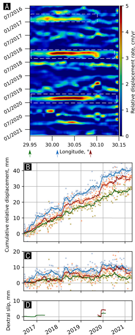
Fig. 3. Spatial and temporal evolution of the East-West relative displacements along the Izmit segment. (A) East-West relative displacement rate along the Izmit segment estimated by using a 50\text{ days} average sliding window, using pixels from 400\text{ m} to 1000\text{ m} away from the fault. The pixels used are shown in Fig. S11. Three high amplitude periods are delimited by white dotted rectangles, corresponding to an increase of relative displacement rates above 4\text{ cm/yr} . The arrows below the figure correspond to the location of the profiles shown on panels (B) and (C), green and red corresponding to the locations of the Izmit and Tepetarla creepmeters, respectively. (B) Cumulative East-West relative displacement estimated at three longitudes, by using pixels from 600\text{ m} -width boxes. The lines correspond to the 60\text{ days} average sliding windows. (C) Corresponding detrended cumulative East-West relative displacement time series obtained after the removal of the linear trend between the transient accelerations. (D) Creepmeter records over the analyzed period of time, green and red corresponding to Izmit and Tepetarla creepmeters, respectively.
