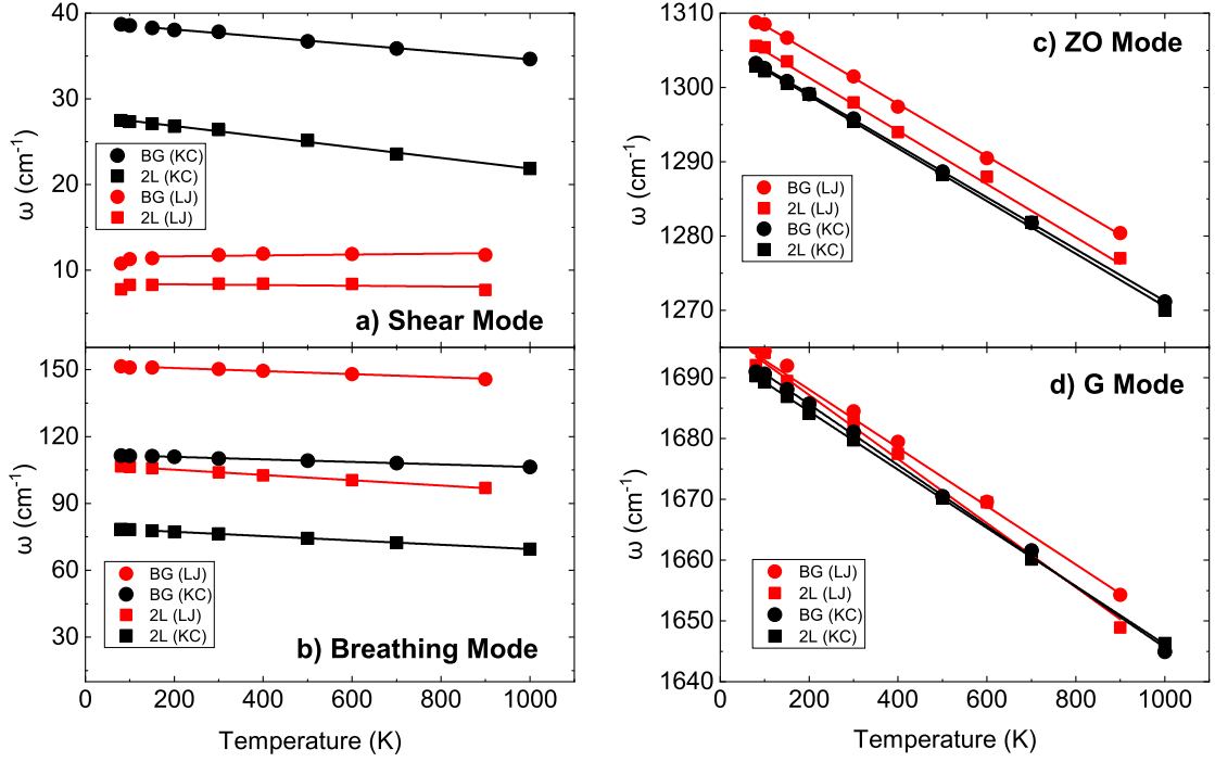
FIG. 6. The calculated temperature dependence \omega(T) of phonon energies for the interlayer (a) Shear (b) Breathing (c) ZO and (d) G mode in 2L (square symbols) and graphite (round symbols), using KC (black full symbols) and LJ (red crossed symbols) as interlayer potentials.
