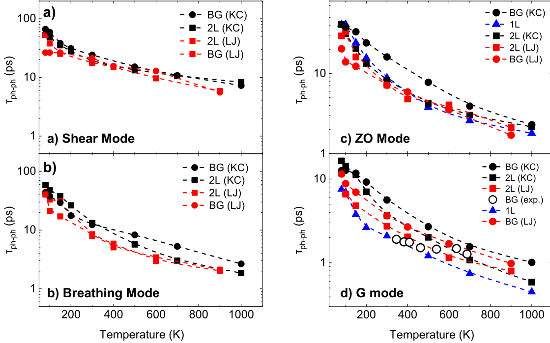
FIG. 7. The calculated temperature dependence \tau^{ph-ph}(T) of phonon lifetimes for the interlayer (a) Shear (b) Breathing (c) ZO and (d) G mode in 2L (square symbols) and graphite (round symbols), using KC (black full symbols) and LJ (red crossed symbols) as interlayer potentials. For the G-mode, the experimental data for graphite from Chatzakis et al [40] are also presented (hollow circles). Dashed lines connecting points are b-splines as visual guides.
