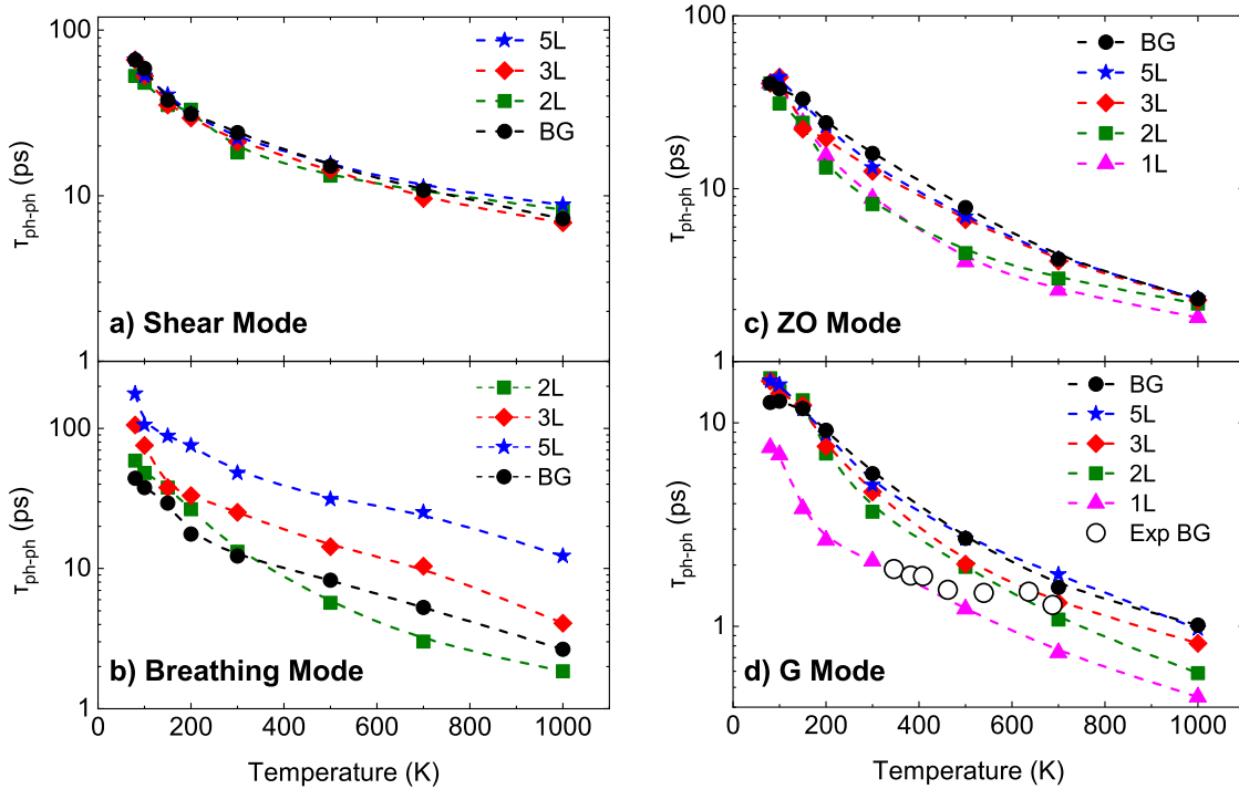
FIG. 4. The calculated temperature dependence of \tau^{ph-ph} of the FLG (a) Shear, (b) Breathing, (c) ZO and (d) G modes with the number of layers N . The correspondence of symbols with N is as follows. 2L: green squares, 3L: red diamonds, 5L: blue stars, BG: black circles. For the G mode, the experimental data from Chatzakis et al [40] are also presented (hollow circles). Dashed lines connecting points are b-splines as visual guides
