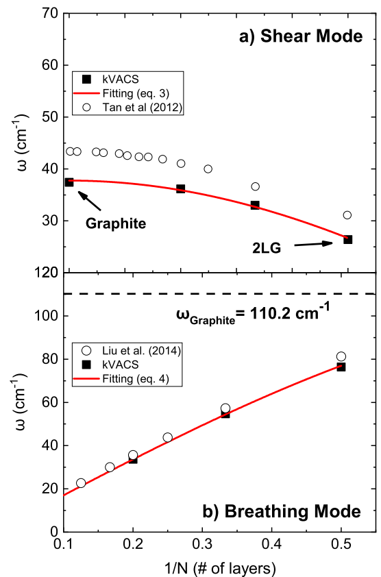
FIG. 2. The calculated dependence of the FLG (a) Shear and (b) Breathing mode at T = 300\text{ K} on the number of layers N (full symbols), along with the fitting of the energies as given by eqs. (3) and (4) (straight line). Experimental measurements by Tan et al. [34] and Lui et al [36] respectively are also shown for comparison (hollow symbols).
