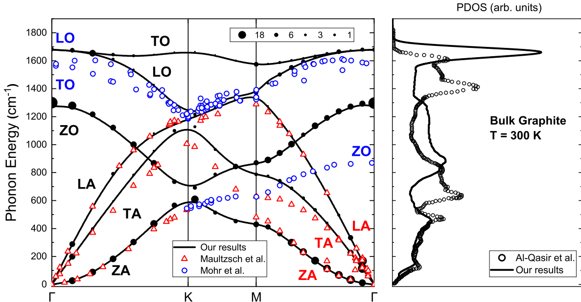
FIG. 1. (Left) The calculated phonon dispersion curves of Bulk Graphite (full symbols) at T = 300 K, together with data from IXS measurements (open symbols) [28, 64]. The magnitude of the kVACS symbols is a measure of the calculated lifetime. Straight lines connecting points are b-splines serving as visual guides. (Right) The calculated phonon DOS for Bulk Graphite at T = 300 K (straight lines), along with data from INS measurements [65] (open symbols). All PDOS are normalized to unit area.
