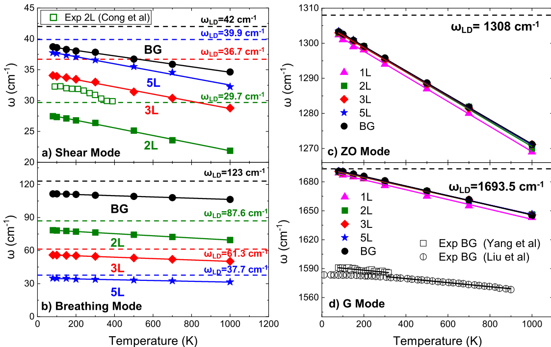
FIG. 3. The calculated temperature dependence of the true FLG (a) Shear (b) Breathing (c) ZO and (d) G phonon mode energies with the number of layers N . The correspondence of symbols with N is as follows. 2L: green squares, 3L: red diamonds, 5L: blue stars, BG: black circles. The hollow symbols represent experimental data by Cong et al [74] Yang et al [75] and Liu et al [76]. The straight lines with the same color correspond to the least-square fittings of the associated data. The dashed lines represent the LD energies for each N .
