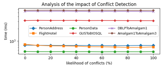
Figure 11: Run-time comparison for different likelihood of conflicts (using CD/PI_NI with 10^5 nodes for each input type).
