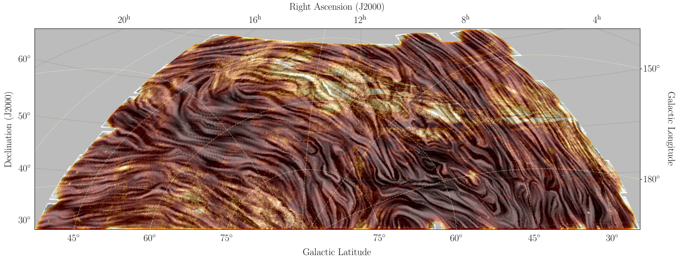
Fig. 5. Magnetic field orientation from Planck at 353 GHz, overlaid on the image of maximum polarised intensity of the LoTSS mosaic.
