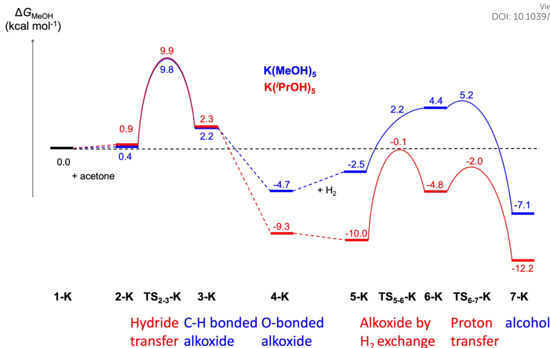
Figure 4. Comparison of the computed Gibbs energy profiles for ketone hydrogenation catalysed by [K(\text{solvent})_5]^+[\text{Ir}(\text{H})_4((\text{S})\text{-P}, \text{S}^{\text{Ph}})]^- with 5 MeOH or 5 i PrOH molecules explicitly included in the calculations.
