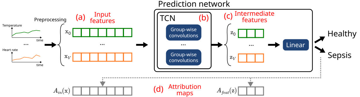
Fig. 1. Overview of the processing pipeline we propose. Preprocessing of raw time series data creates V hour-binned input features \mathbf{x} \in \mathbb{R}^D (a) with D the window size, which are then processed with a TCN model (b) to generate V intermediate feature vectors \mathbf{z} \in \mathbb{R}^d of dimensionality d (c). Our proposed modification on the TCN convolutions allows generating variable-wise attribution maps (d) from both input features A_{in}(\mathbf{x}) \in \mathbb{R}^D and intermediate feature vectors A_{feat}(\mathbf{z}) \in \mathbb{R}^d .
