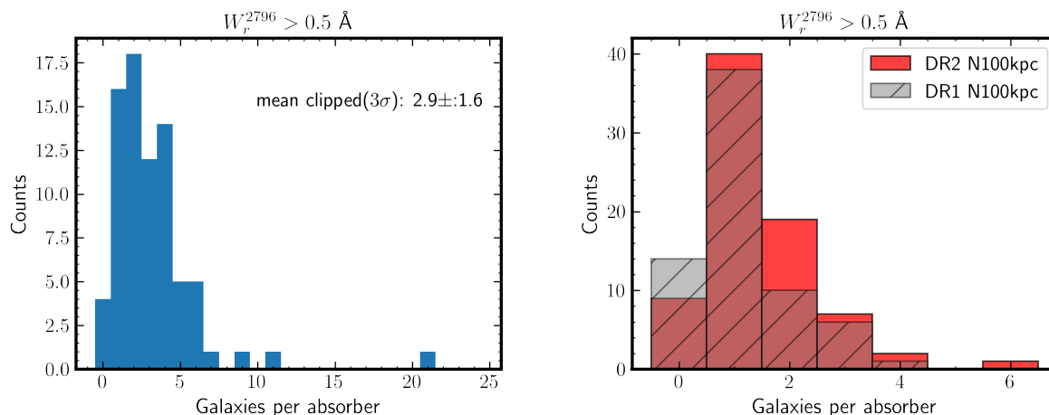
Fig. 9: Left : Distribution of the number of galaxies that are within \pm 500 \text{ km s}^{-1} of strong ( W_r^{2796} > 0.5 \text{ \AA} ) absorption systems, within the MUSE FOV, and within the MUSE wavelength coverage for [O II] emitters, i.e. 0.35 < z_{\text{abs}} < 1.45 . The mean (median) number of galaxies is 2.9 \pm 1.6 (3.0), respectively. Right : The red (hashed) histogram shows the number of galaxies around strong ( W_r^{2796} > 0.5 \text{ \AA} ) Mg II absorption systems within 100 kpc in the redshift range 0.35 < z < 1.45 suitable for [O II] emitters, from the DR2 (DR1) samples, respectively.
