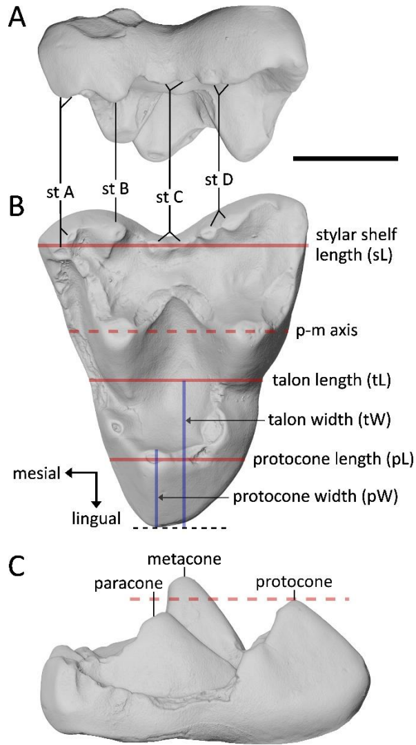
Figure 3. Measurement methods of mesiodistal length (sL, tL, pL) and labiolingual width (tW, pW) of peratheriine upper molars introduced in this study, with the positioning of styler cusps and main cusps, illustrated on the left M3 MNHN.F.CB1252, Peratherium maximum comb. nov. from Condé-en-Brie (~MP8+9, Paris Basin), in labial (A), occlusal (B), and mesial (C) views. The arrows indicating the mesial and lingual sides concern the occlusal view (B). The red dashed line in the mesial view (C) is used to compare the heights of the main cusps. Scale bar equals 1 mm. Abbreviations: p-m axis, paracone – metacone axis; st, styler cusp.
