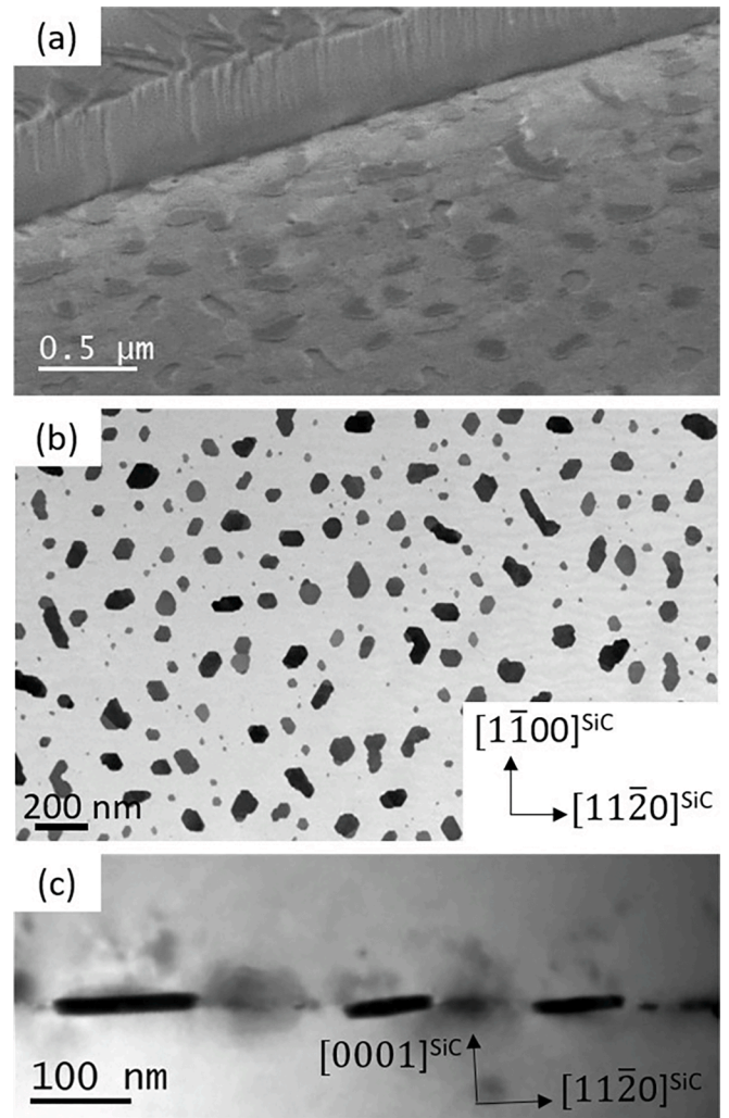
Fig. 1. SEM, STEM and TEM images of the SiC/2 nm W/SiC structure annealed at 1900^\circ\text{C} for 30 min: (a) 52^\circ -tilted SEM image of the interface once the top substrate has been removed by cleavage; (b) Bright-field plan view STEM image; (c) Bright-field cross-sectional (1\bar{1}00) TEM image of the nodules.
