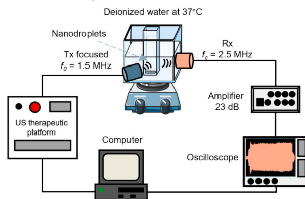
Fig. 1. Nanodroplet acoustic characterization: A - Detection of nanodroplet vaporization threshold using an inverted optical microscope and high-speed camera. B - Acoustic signature characterization device for nanodroplets.
