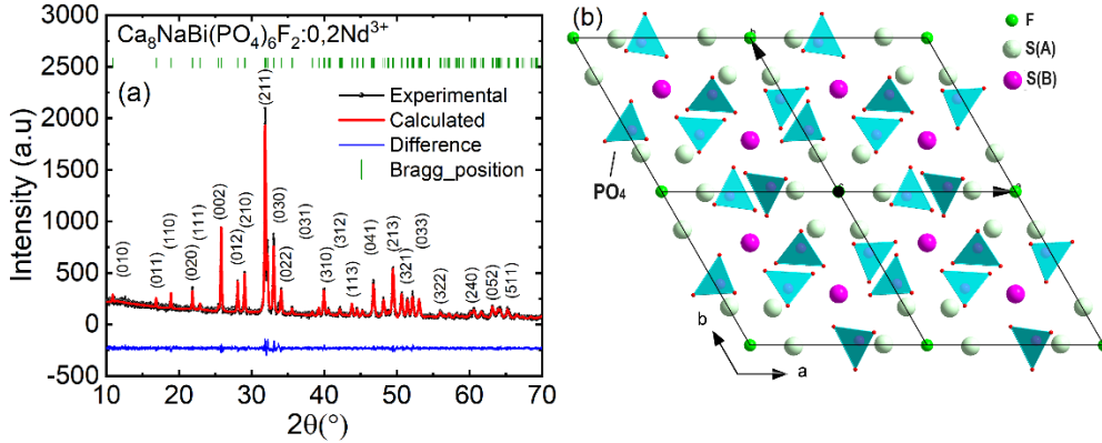
Figure 3. (a) Rietveld refinement of the XRD pattern of the sample \text{Ca}_8\text{NaBi}(\text{PO}_4)_6\text{F}_2:0.2\text{Nd}^{3+} ; experimental ( black ), calculated ( red ) and differential ( blue ) profiles and Bragg reflections ( green dashes ), ( hkl ) are the Miller's indices; (b) projection of the crystalline structure of \text{Ca}_8\text{NaBi}(\text{PO}_4)_6\text{F}_2:\text{Nd} on the a - b plane.
