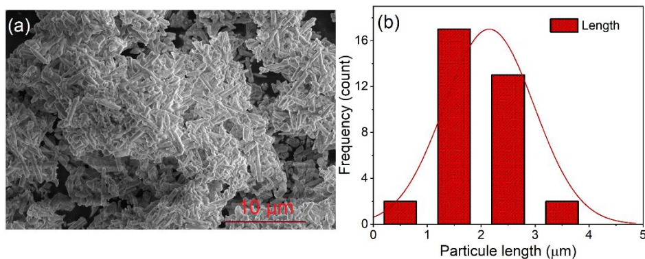
Figure 5. (a) A typical SEM image and (b) the corresponding particle size distribution for the \text{Ca}_8\text{NaBi}(\text{PO}_4)_6\text{F}_2:0.2\text{Nd} phosphor.
