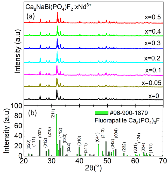
Figure 2. (a) X-ray powder diffraction (XRD) patterns of the \text{Ca}_8\text{NaBi}(\text{PO}_4)_6\text{F}_2:x\text{Nd}^{3+} phosphors with x = 0, 0.05, 0.1, 0.2, 0.3, 0.4 and 0.5 ; (b) theoretical pattern for fluorapatite, JCPDS card # 96-900-1879.
