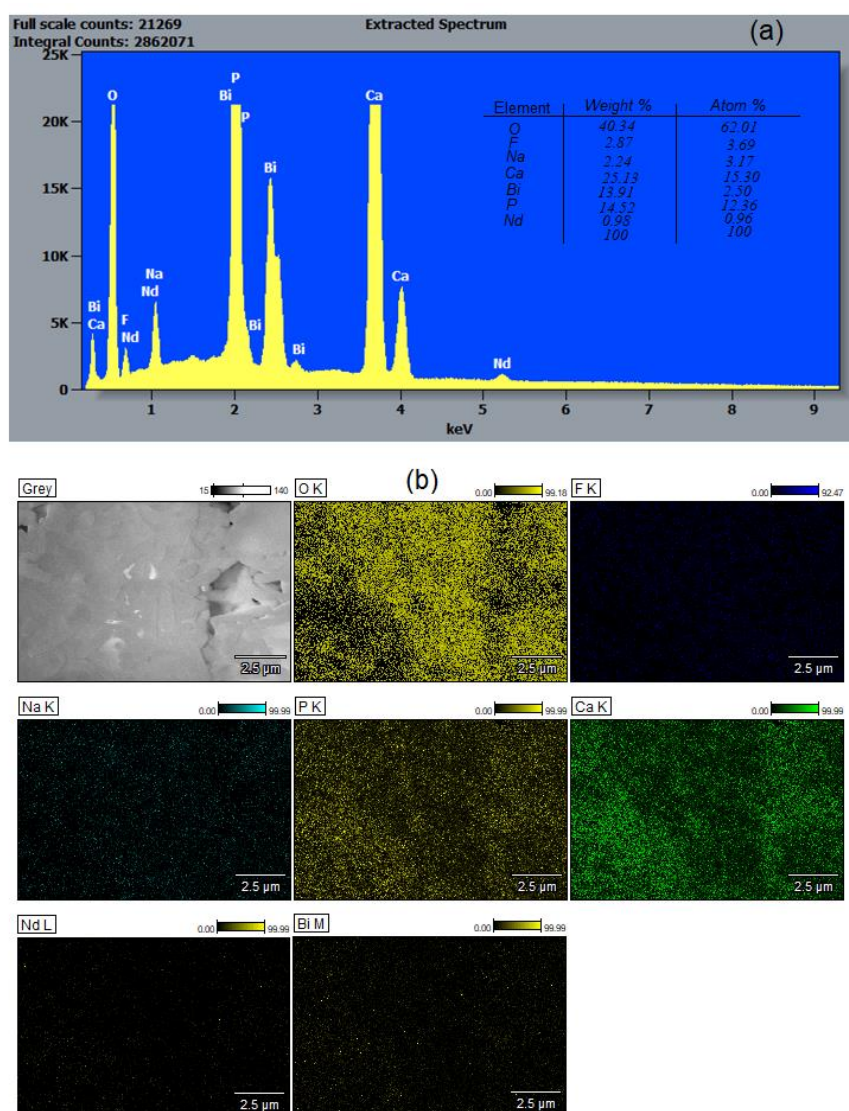
Figure 6. (a) A typical Energy-Dispersive X-ray (EDX) spectrum of the \text{Ca}_8\text{NaBi}(\text{PO}_4)_6\text{F}_2:0.2\text{Nd} sample; (b) the corresponding SEM image and element maps (O, F, Na, P, Ca, Nd and Bi).
