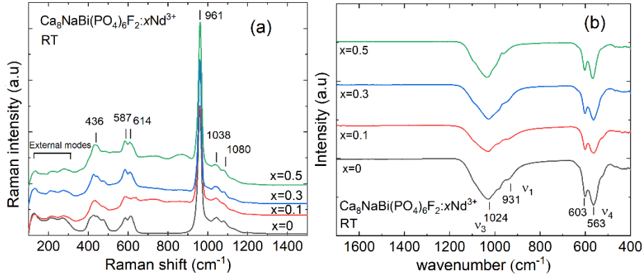
Figure 4. (a) Raman and (b) IR spectra of the \text{Ca}_8\text{NaBi}(\text{PO}_4)_6\text{F}_2:x\text{Nd} samples for x = 0, 0.1, 0.3 and 0.5 .
