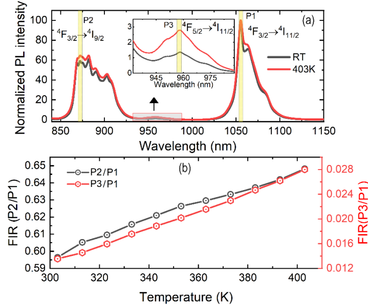
Figure 10. Thermometry performance characterizations: (a) Normalized photoluminescence emission spectra of the \text{Ca}_8\text{NaBi}(\text{PO}_4)_6\text{F}_2:0.2\text{Nd}^{3+} microrods measured at room temperature (303 K) and 403 K upon 808 nm laser excitation; (b) Plot of FIRs P2/P1 and P3/P1 as a function of temperature (303 – 403 K); P1 at 1055 nm, P2 at 872 nm and P3 at 957 nm.
