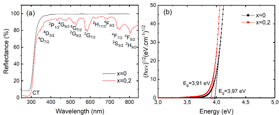
Figure 7. (a) Reflectance spectra of the host matrix and the \text{Ca}_8\text{NaBi}(\text{PO}_4)_6\text{F}_2:0.2\text{Nd}^{3+} sample and (b) Tauc plot to assess the optical band gap energy.
