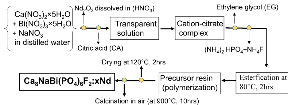
Figure 1. Illustration depicting the modified Pechini synthesis of the \text{Ca}_8\text{NaBi}(\text{PO}_4)_6\text{F}_2:x\text{Nd}^{3+} phosphors.
