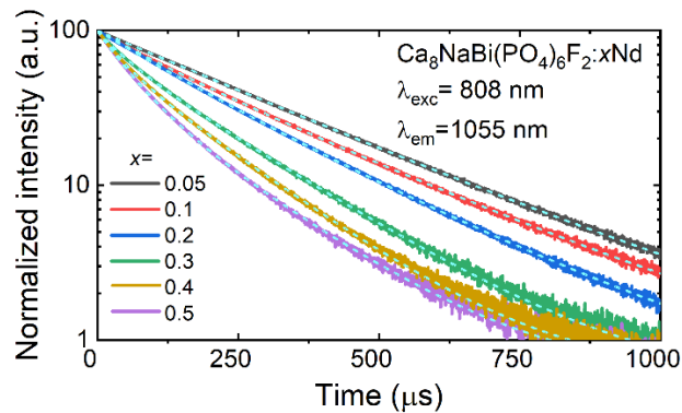
Figure 9. Luminescence decay curves for the {}^4\text{F}_{3/2} state of \text{Nd}^{3+} ions in the \text{Ca}_8\text{NaBi}(\text{PO}_4)_6\text{F}_2:x\text{Nd} phosphors with x = 0.05, 0.1, 0.2, 0.3, 0.4 and 0.5 ; \lambda_{\text{lum}} = 1055 nm and \lambda_{\text{exc}} = 808 nm; dashed lines are the exponential fit.
