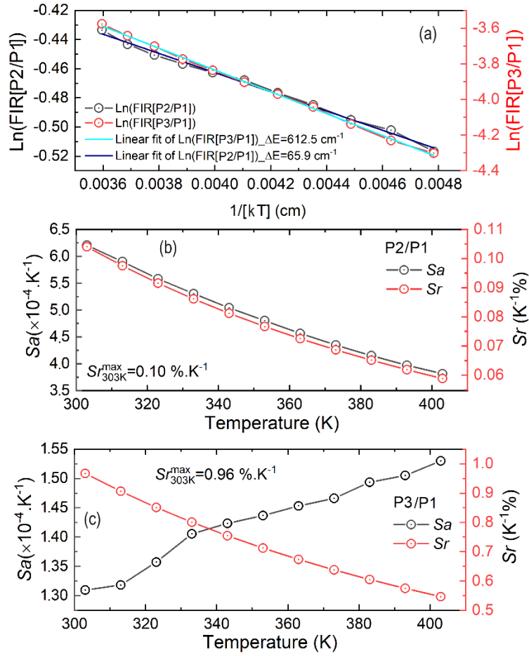
Figure 11. Thermometry performance characterizations: (a) linear fitting of \ln(\text{FIR}) as function of 1/[kT] ; Variation of the relative sensitivity ( Sr ) and the absolute sensitivity ( Sa ) as function of the temperature (303 – 403 K): (b) from the FIR P2/P1; (c) from the FIR P3/P1; P1 at 1055 nm, P2 at 872 nm and P3 at 957 nm.
