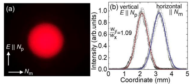
Fig. 6. Spatial characteristics of red emission from the Sm:KGD(WO 4 ) 2 laser: (a) A photograph of the laser beam in the far-field; (b) 1D intensity profiles (symbols – experimental data, curves – Gaussian fits). T_{oc} = 0.1\% .
