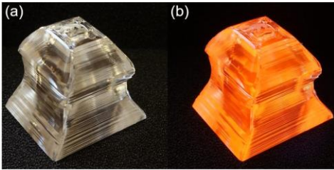
Fig. 1. A photograph of an as-grown 0.4 at.% \text{Sm}:\text{KGd}(\text{WO}_4)_2 crystal (the growth direction is along the [010] axis): (a) Natural light; (b) Under UV illumination.
