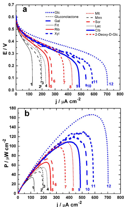
Figure 4. Representative EFC performances recorded in a slightly stirred citrate/phosphate buffer (0.2 M, pH 6.5) containing different saccharides (50 mM). Fuel cell polarizations in terms of: (a) cell voltage E and (b) power density P . The polarization curves are recorded by sweeping the current at 0.2 \mu\text{A s}^{-1} from zero until short circuit ( E = 0 ), in a non-compartmentalized cell and without any external addition of O 2 . Note: 1 = Frt (fructose), 2 = Mnn (mannose), 3 = gluconolactone, 4 = Lac (lactose), 5 = Rib (ribose), 6 = Scr (sucrose), 7 = 2-Deoxy-D-glc (2-deoxy-D-glucose), 8 = Mlt (maltose), 9 = Clb (cellobiose), 10 = Gal (galactose), 11 = Xyl (xylose), 12 = Glc (glucose).
