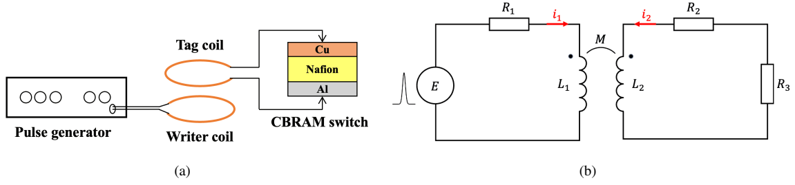
Figure 3. (a) Proposed writing circuit. (b) Equivalent circuit of the writing circuit.
