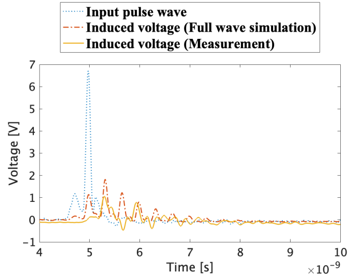
Figure 7. Input pulse voltage and induced voltage using simulated s2p and measured s2p.
