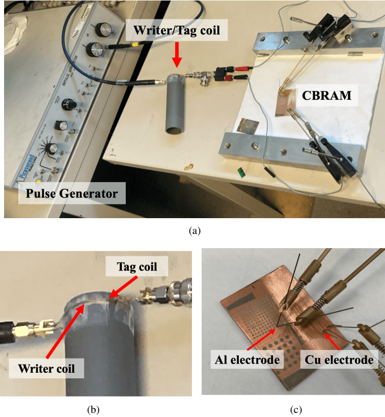
Figure 9. (a) Experimental environment. (b) Implemented coils. (c) CBRAM used in experiments.
