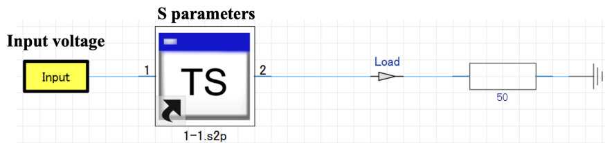
Figure 6. Schematic of a circuit simulation to calculate induced voltage at the CBRAM terminals.
