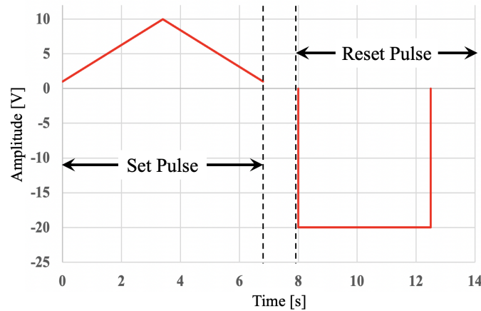
Figure 2. Direct current (DC) pulses used with CBRAM cells in a classical writing method [7].
