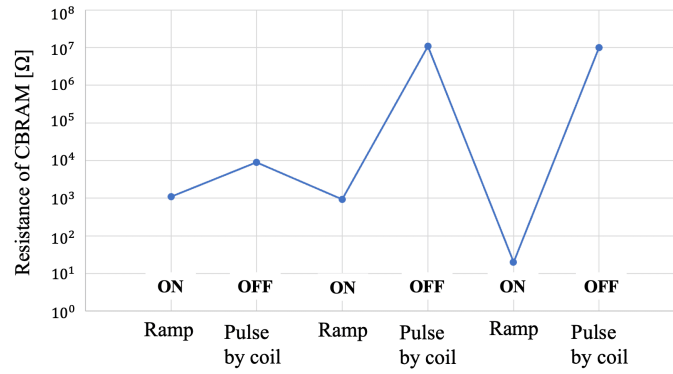
Figure 10. Switching results of CBRAM with pulse waves.
