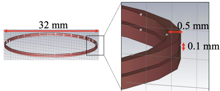
Figure 4. Coil models in CST.
