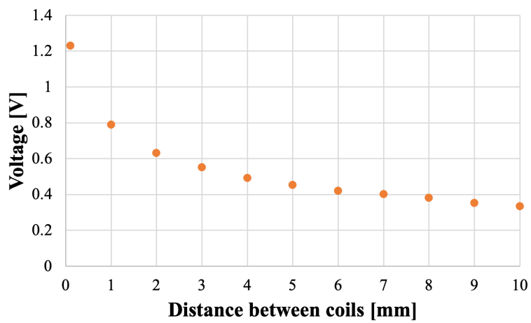
Figure 8. Peak of the induced voltage (CBRAM terminal) when changing the distance between coils.
