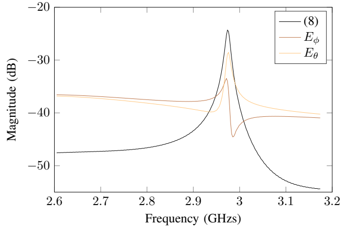
Fig. 30. Simulated S-parameters on a loop resonator with \alpha_y = 45^\circ with an incoming wave excitation along E_\theta and \theta = \phi = 80^\circ .
