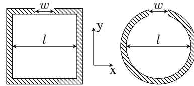
Fig. 33. Square and circular resonator topology.
