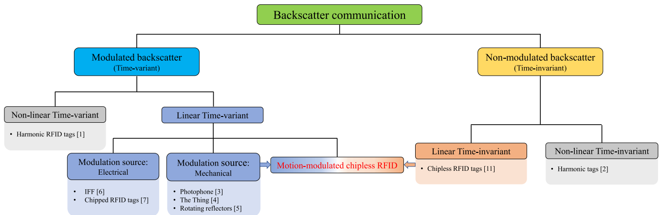
FIGURE 1. Classification of backscatter communication methods.
