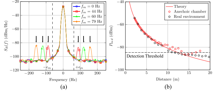
FIGURE 11. (a) Measured PSD of the backscattered signal from polarization-modulated chipless tag for different rotational speed. Sensing is realized based on the frequency position of the side lobes. (b) Differential backscattered power as a function of distance [34].
