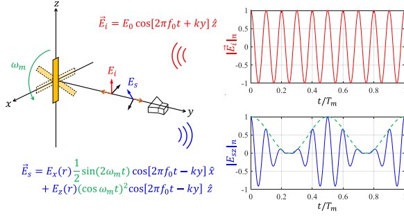
FIGURE 9. Polarization-modulated chipless tag. The normalized magnitude of the incident and scattered field is shown as a function of time during one period of motion ( T_m = 2\pi/\omega_m ) respectively in red and blue color. The amplitude modulating waveform induced by the motion is also shown for better interpretation with dashed green line.
