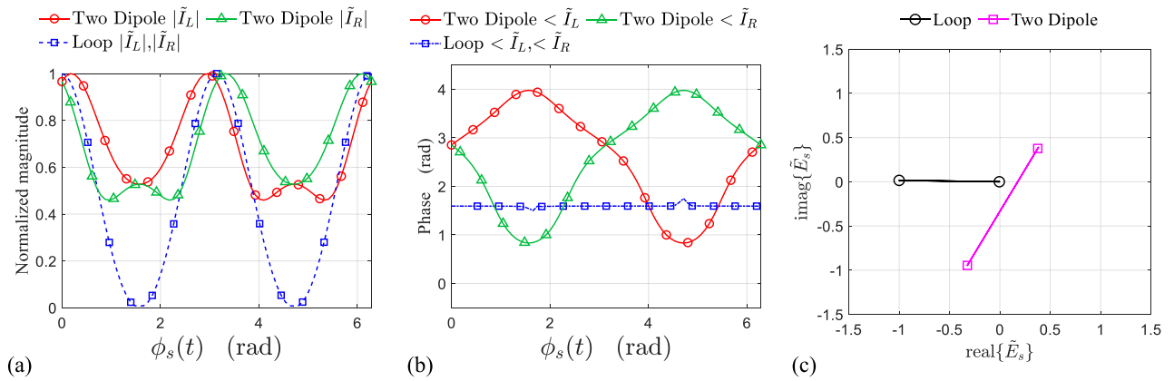
Figure 6. (a) Normalized magnitude, (b) phase of left-side and right-side induced currents on the two symmetrically rotating dipoles and the rectangular loop. (c) IQ constellation of the time-varying complex envelope of the normalized backscattered field from symmetrically rotating loop and two symmetrically rotating dipole. All the data are obtained in simulation.
