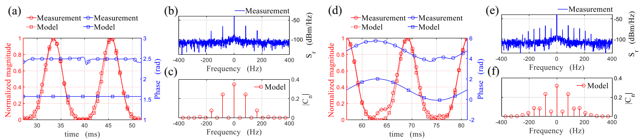
Figure 9. The magnitude and phase of the measured amplitude modulating waveform for (a) symmetrical, (d) non-symmetrical rotation of the loop compared with those predicted by the model. The measured PSD of the received signal backscattered from (b) symmetrically, (e) non-symmetrically rotating loop. The calculated Fourier coefficients of the time-varying complex envelope of the backscattered field from (c) symmetrically, (f) non-symmetrically rotating loop.
