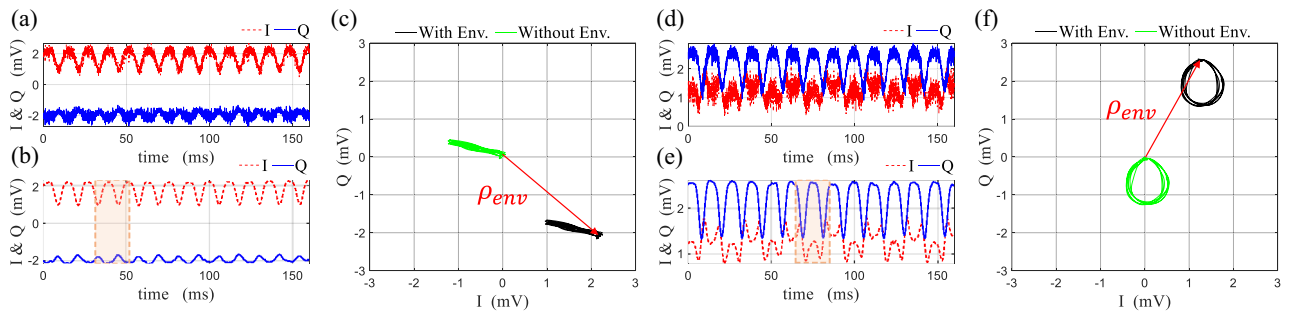
Figure 7. Obtained raw IQ data in measurement for scattering from (a) symmetrically, (d) non-symmetrically rotating rectangular loop, and the averaged IQ data for scattering from (b) symmetrically (e) non-symmetrically rotating rectangular loop. The measured IQ constellation plotted based on the averaged data for (c) symmetrically (f) non-symmetrically rotating rectangular loop. The original measured modulation paths are shown in black color, and after the subtraction of the environment contribution (red arrow) they are shown in green color.
