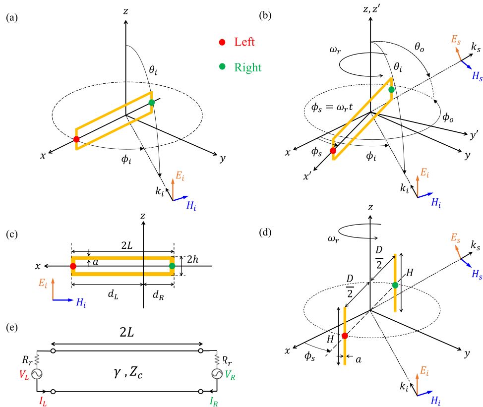
Figure 3. (a) Non-symmetrically positioned rectangular loop impinged by vertically polarized plane wave. (b) Scattering from non-symmetrically rotating rectangular loop. (c) Geometrical dimensions of the rectangular loop. (d) Scattering from two symmetrically rotating coupled dipoles. The left and right side radiating elements are respectively remarked with red and green dots. (e) The proposed circuit model for the wave-impinged loop.
