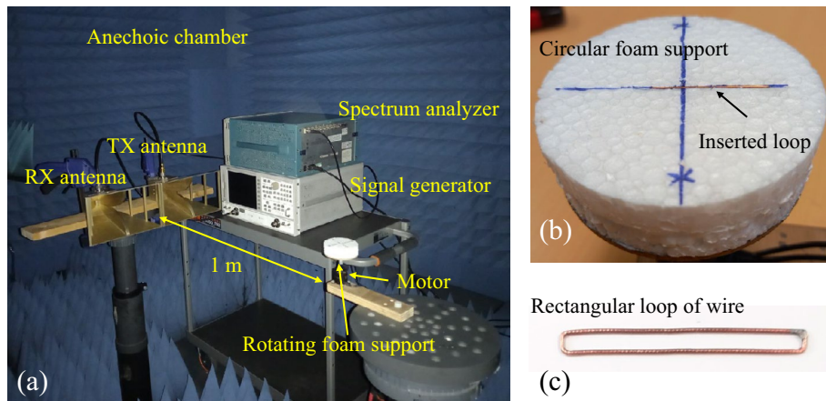
Figure 11. (a) The measurement bench in the anechoic chamber. (b) The circular foam support used for rotating the rectangular loop. (c) Fabricated rectangular loop.
