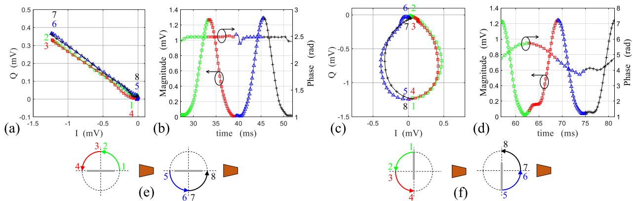
Figure 8. The modulation path during one period of rotation for (a) symmetrically, (c) non-symmetrically rotating loop. The magnitude and phase variation of the retrieved modulating waveform from measured signal for (b) symmetrically, (d) non-symmetrically rotating loop during one period of rotation. Each period of rotation is divided to four sections shown in green, red, blue and black color on the modulation path and modulating waveform. The respective orientation of the loop is given at each section for (e) symmetrical, (f) non-symmetrical rotation.
