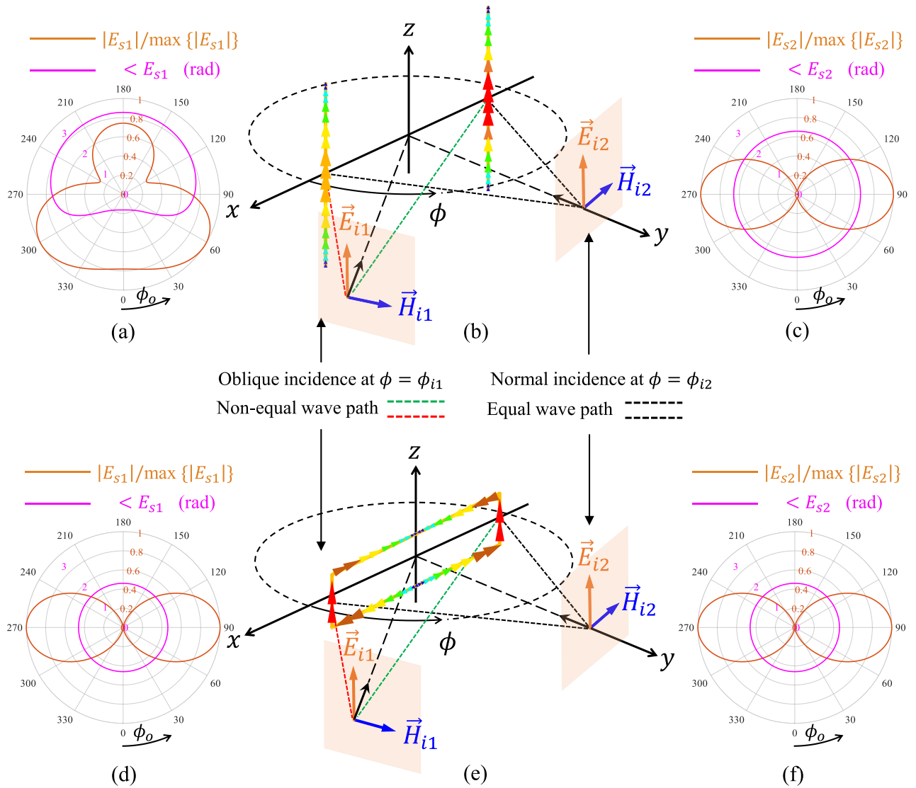
Figure 1. The azimuth distribution ( 0^\circ < \phi_o < 360^\circ ) of the phase and normalized magnitude of the scattered electric field from two dipoles for (a) oblique incidence (c) normal incidence. The azimuth distribution ( 0^\circ < \phi_o < 360^\circ ) of the phase and normalized magnitude of the scattered electric field from rectangular loop for (d) oblique incidence (f) normal incidence. Symmetrical and non-depolarizing scattering structure (b) without radial resonance [two equal-length coupled dipoles] (e) with radial resonance [rectangular loop]. All the data are obtained in simulation.
