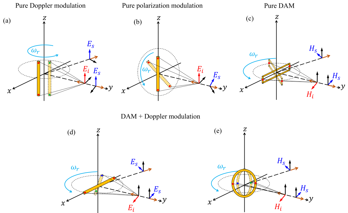
Figure 10. Backscatter communication based on rotating scatterers with (a) pure Doppler modulation, (b) pure polarization modulation, and (c) pure DAM. (d,e) backscatter communication with combined DAM and Doppler modulation. The phase change of the induced current on the scatterer during the rotation in (d,e) is shown by two red dots for normal incidence, and one blue and one green dot for oblique incidence.
