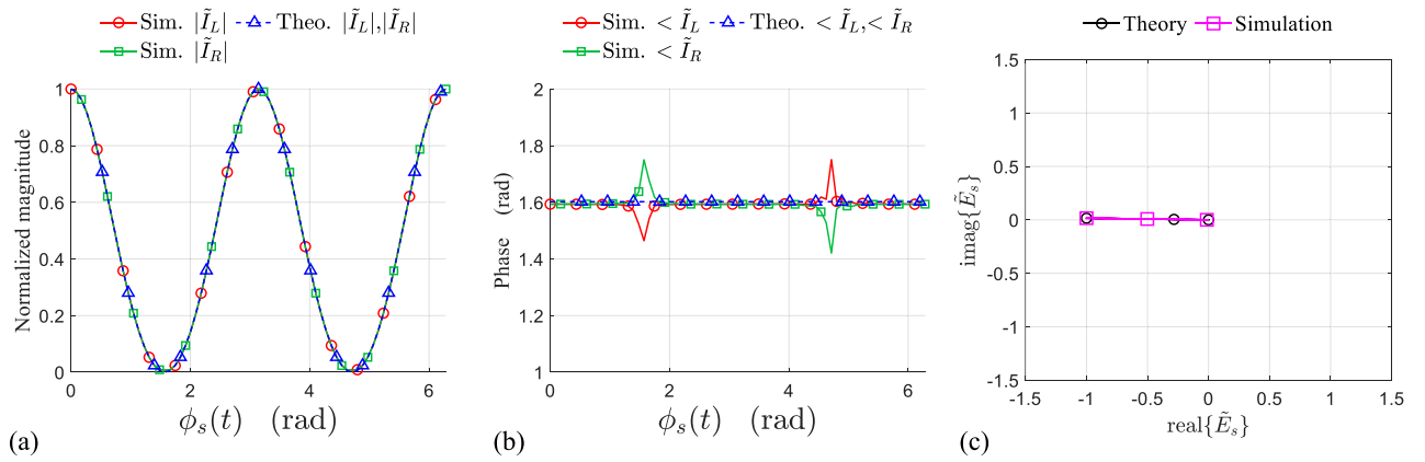
Figure 4. (a) Normalized magnitude, (b) phase of the induced currents on the left and right side of the symmetrically rotating rectangular loop during one period of rotation, obtained from the model and simulations. (c) IQ constellation of the time-varying complex envelope of the normalized backscattered field from symmetrically rotating loop in simulation and theory.
