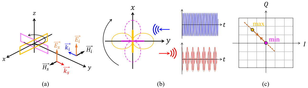
Figure 2. (a) Rotating rectangular loop in the monostatic scattering configuration. (b) Directional amplitude modulation induced on the backscattered wave by rotating loop. (c) The IQ constellation diagram of the demodulated received signal. The linear modulation path crosses the origin, and is limited in between the minimum and maximum of the reradiation pattern corresponding to the positions of the loop shown in (b).
