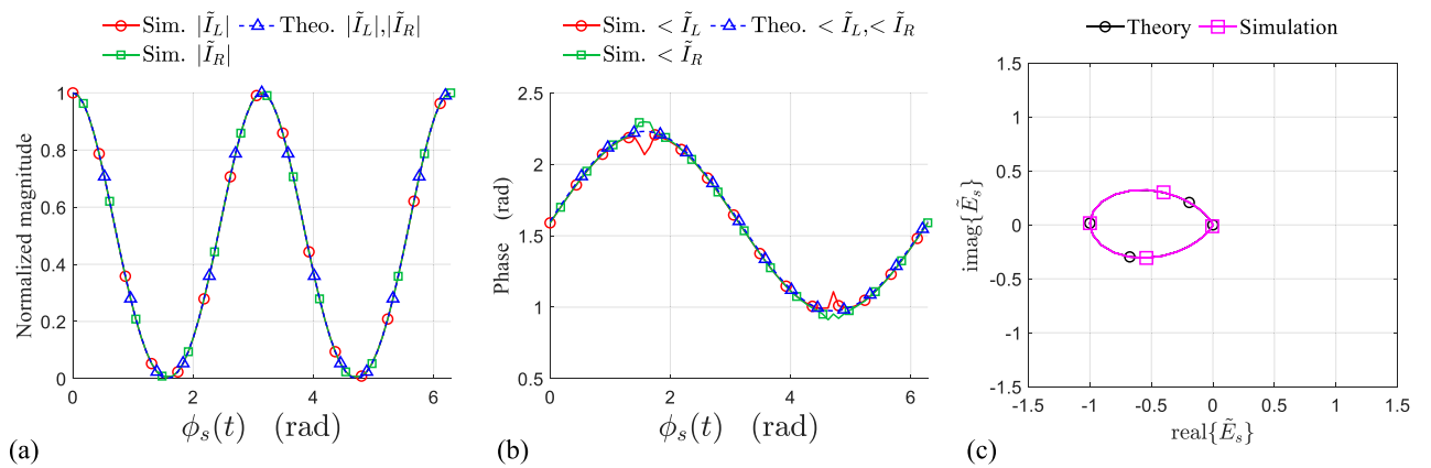
Figure 5. (a) Normalized magnitude, (b) phase of the induced currents on the left and right side of the non-symmetrically rotating rectangular loop during one period of rotation, obtained from the model and simulations. (c) IQ constellation of the time-varying complex envelope of the normalized backscattered field from non-symmetrically rotating loop in simulation and theory.
