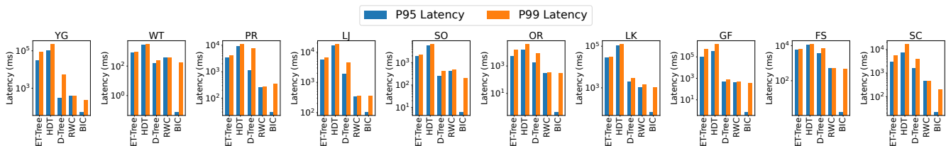
Figure 8: P95 and P99 tail latency analysis using windows of on average 3M edges and slide intervals of on average 150K edges.
