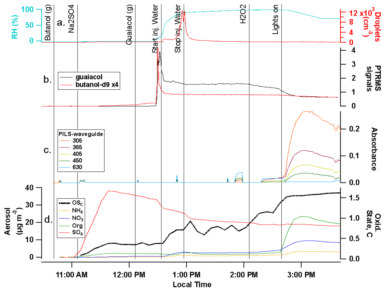
Figure 1: Experiment 3. Na 2 SO 4 seeds, guaiacol, cloud event, and HOOH + lights. Panel a : RH (blue line) and droplet counts (red, right axis). b : PTR-MS signals for guaiacol (black line) and butanol- d 9 (red, multiplied by a factor of 4). c : absorbance measured in water-soluble aerosol particles by PILS / waveguide UV-vis, with absorbance below detection limit shown as flat baseline. d : average oxidation state of carbon (black line) and ACSM aerosol loadings after
