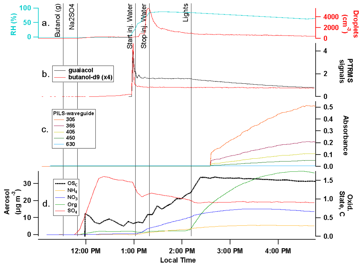
Figure 2: experiment 4 with \text{Na}_2\text{SO}_4 seed particles, gas-phase guaiacol, a cloud event, and simulated sunlight, but no \text{HOOH} . Panel a : RH (blue line) and droplet counts (red, right axis). b : PTR-MS signals for guaiacol (black line) and butanol- d_9 (red, multiplied by a factor of 4). c : absorbance measured in water-soluble aerosol particles by PILS / waveguide UV-vis, with absorbance below detection limit shown as flat baseline. d : average oxidation state of carbon (black line) and ACSM aerosol loadings after dilution corrections, for sulfate (red), organic (green), nitrate (blue), and ammonium-assigned signals (orange).
