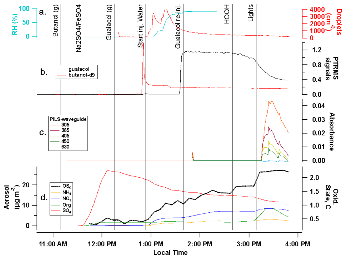
Figure 5: Experiment 8. Photo-Fenton chemistry aerosol experiment with \text{Na}_2\text{SO}_4 / \text{FeSO}_4 seeds, guaiacol, high RH, and \text{HOOH} + \text{lights} . Panel a : RH% (blue line) and droplet counts (red, right axis). b : PTR-MS signals for guaiacol (black line) and butanol- d9 (red). c : absorbance measured in water-soluble aerosol particles by PILS / waveguide UV-vis, with absorbance below detection limit shown as flat baseline. d : average oxidation state of carbon (black line) and ACSM aerosol loadings after dilution corrections, for sulfate (red), organic (green), nitrate (blue), and ammonium-assigned signals (orange).
