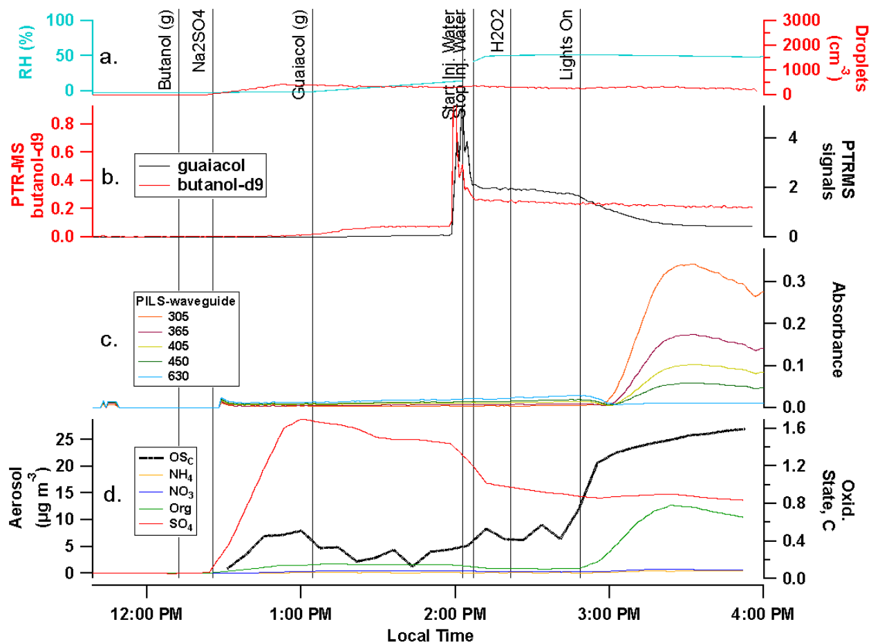
Figure 4: Experiment 5, performed at 50% RH with undeliquesced \text{Na}_2\text{SO}_4 seeds, guaiacol, and \text{HOOH} + lights. Panel a : RH (blue line) and droplet counts (red, right axis). b : PTR-MS signals for guaiacol (black line) and butanol- d_9 (red, left axis). c : absorbance measured in water-soluble aerosol particles by PILS / waveguide UV-vis, with absorbance below detection limit shown as flat baseline. d : average oxidation state of carbon (black line) and ACSM aerosol loadings after dilution corrections, for sulfate (red), organic (green), nitrate (blue), and ammonium-assigned signals (orange).
