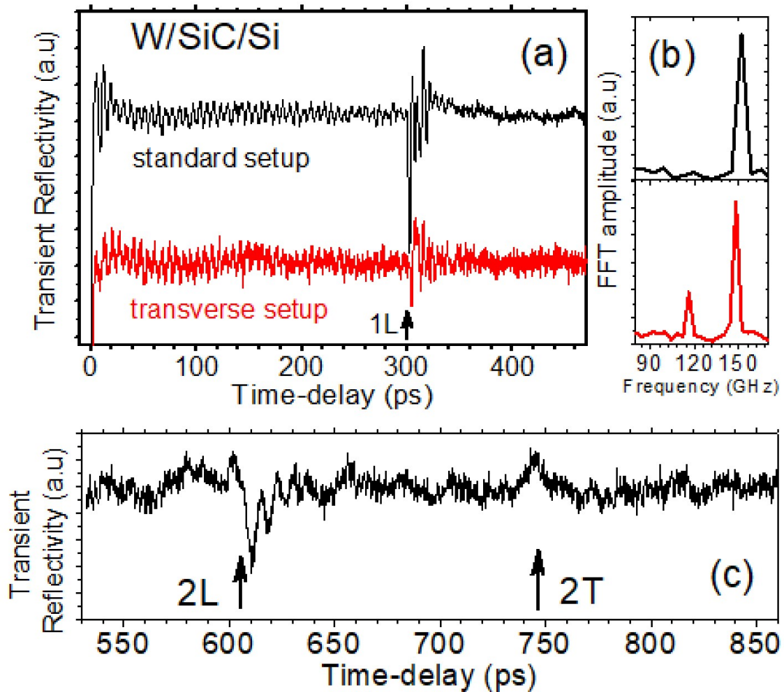
Figure 3 – (a) Transient relative reflectivity change in W/SiC/Si sample measured with two distinct setups: standard means normal incidence with no sensitivity to polarization change; transverse setup means probe incidence at 45^\circ with an optical detection sensitive to change in light polarization. (b) Fourier Transform of the transient reflectivity change. (c) Transient signal measured at longer time-delays: 2L (resp. 2T) is identified as the round-trip of the longitudinal (resp. transverse) pulse.
