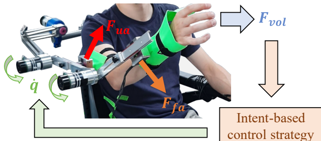
Fig. 1: Usability of the proposed intent-based controller is assessed with a prototype of an UL assistive exoskeleton. User intent is detected by retrieving voluntary forces ( F_{vol} ) from interaction forces ( F_{ua} , F_{fa} ) and translated to actuator velocities ( \dot{q} ) with an intent-based control strategy.
