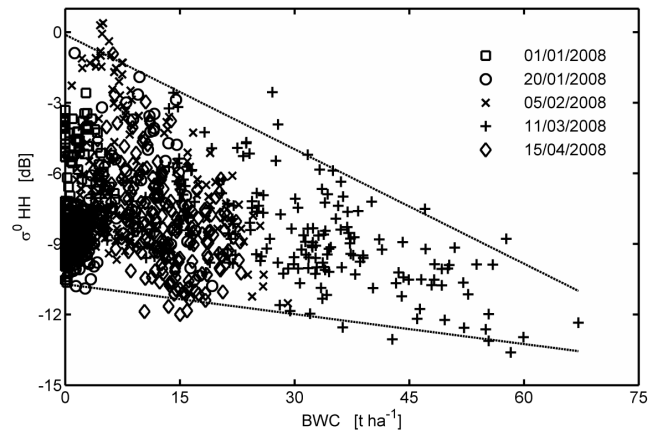
Fig. 7. Backscattering coefficients ( \sigma^0_{HH} ) versus biomass water content (BWC) for ASAR images acquired in ascending orbit and incidence angle IS1. Each symbol corresponds to one satellite over-pass. The wet (top) and dry (bottom) lines are displayed.
