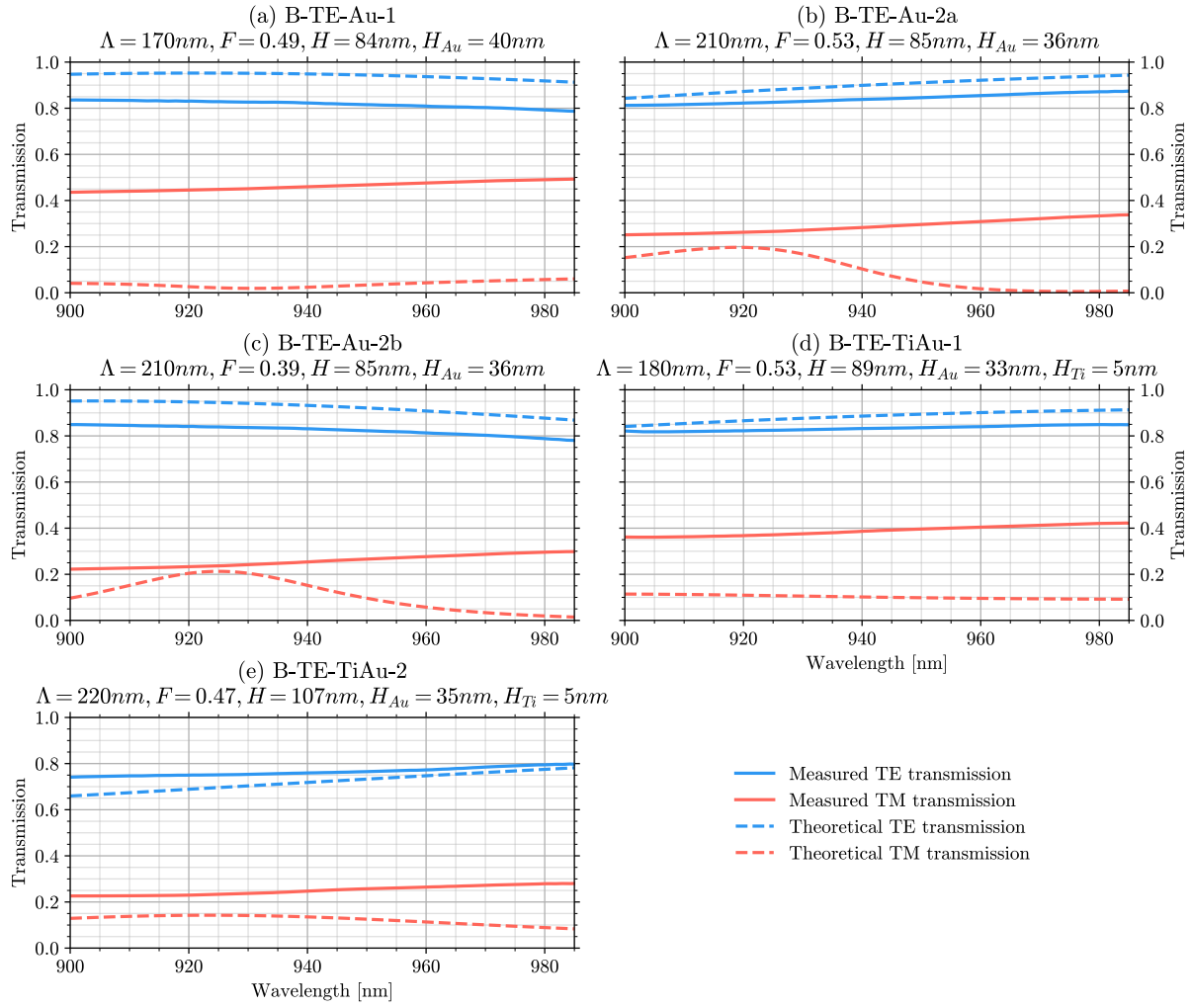
Figure 5: Comparison between measured and calculated spectral transmission of different fabricated B-TE MetalMHCs at normal incidence between 900 and 985 nm. For each structure, the grating dimensions are specified : the period \Lambda , the fill-factor F , the gallium arsenide height H , the gold height H_{Au} , and the titanium height H_{Ti} .
